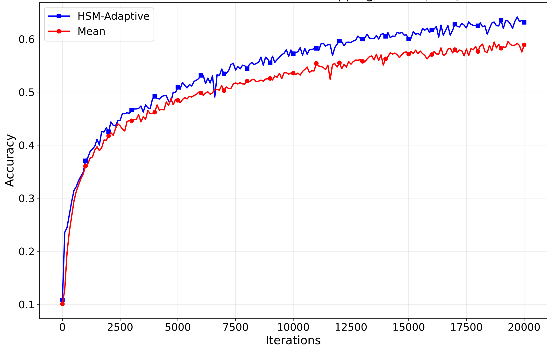
CIFAR-10 - IID Partition - Label Flipping Attack (b=3)
