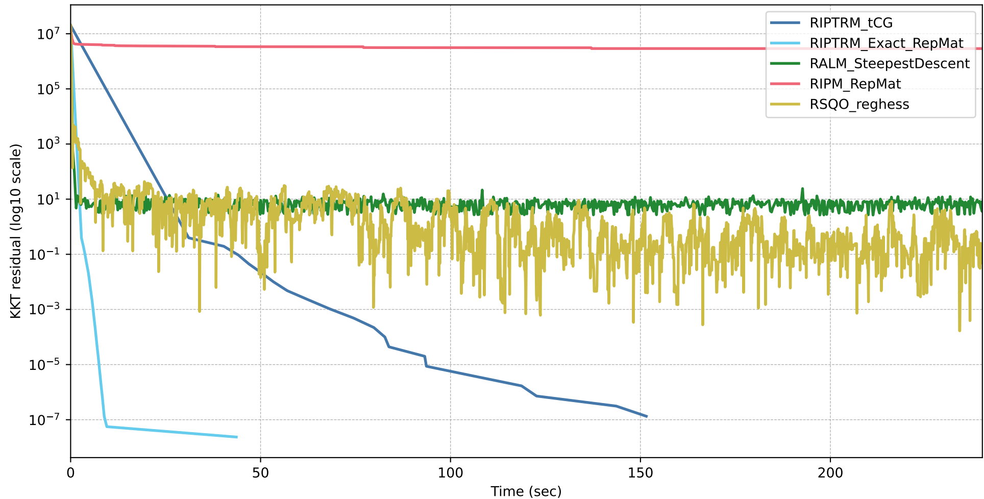
time vs residual for Rosenbrock-1-a
