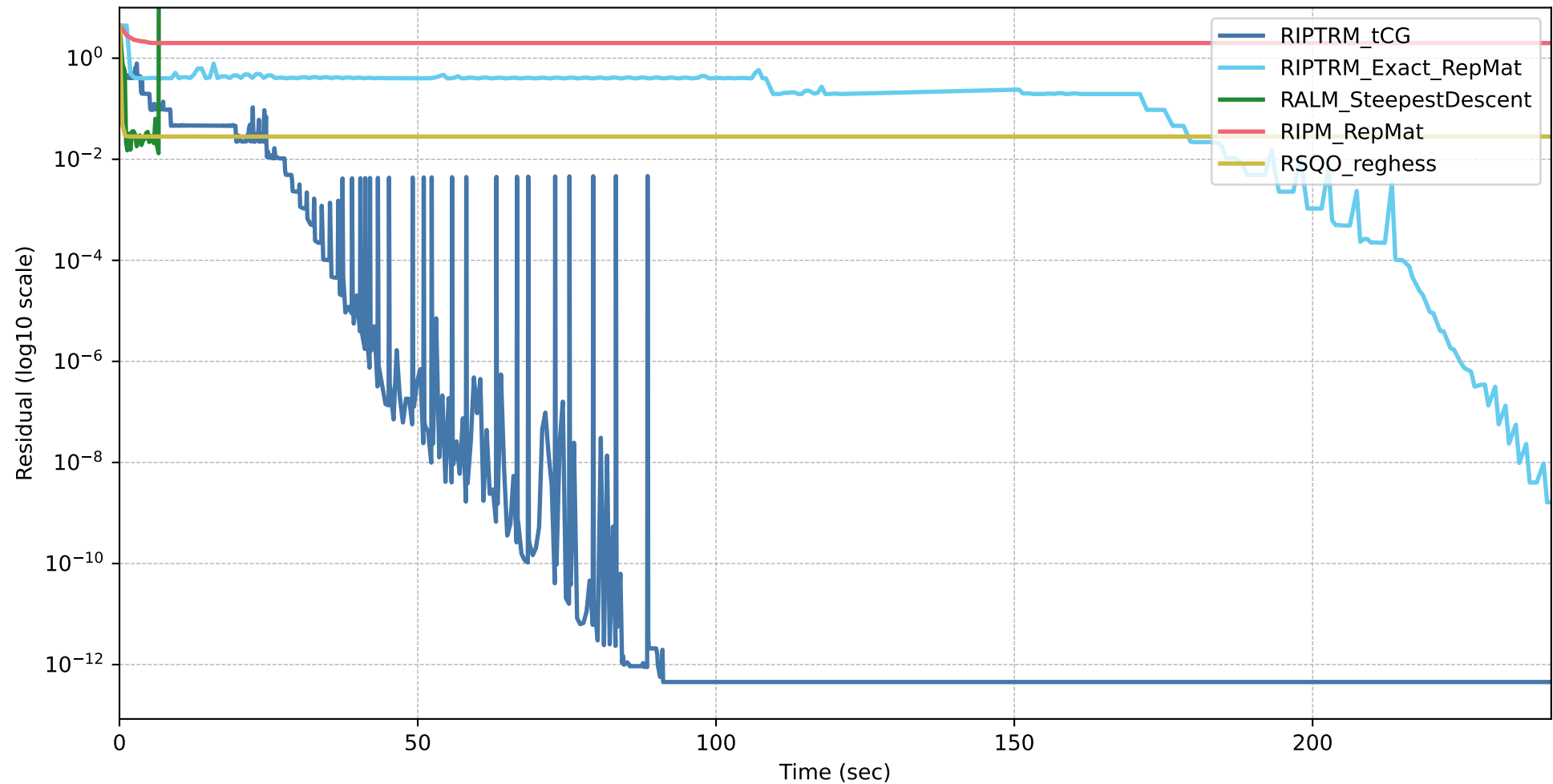
time vs residual for StableIdentification-1-r
