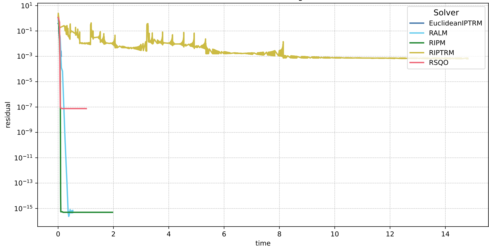
time vs residual for NonnegPCA-1-a
