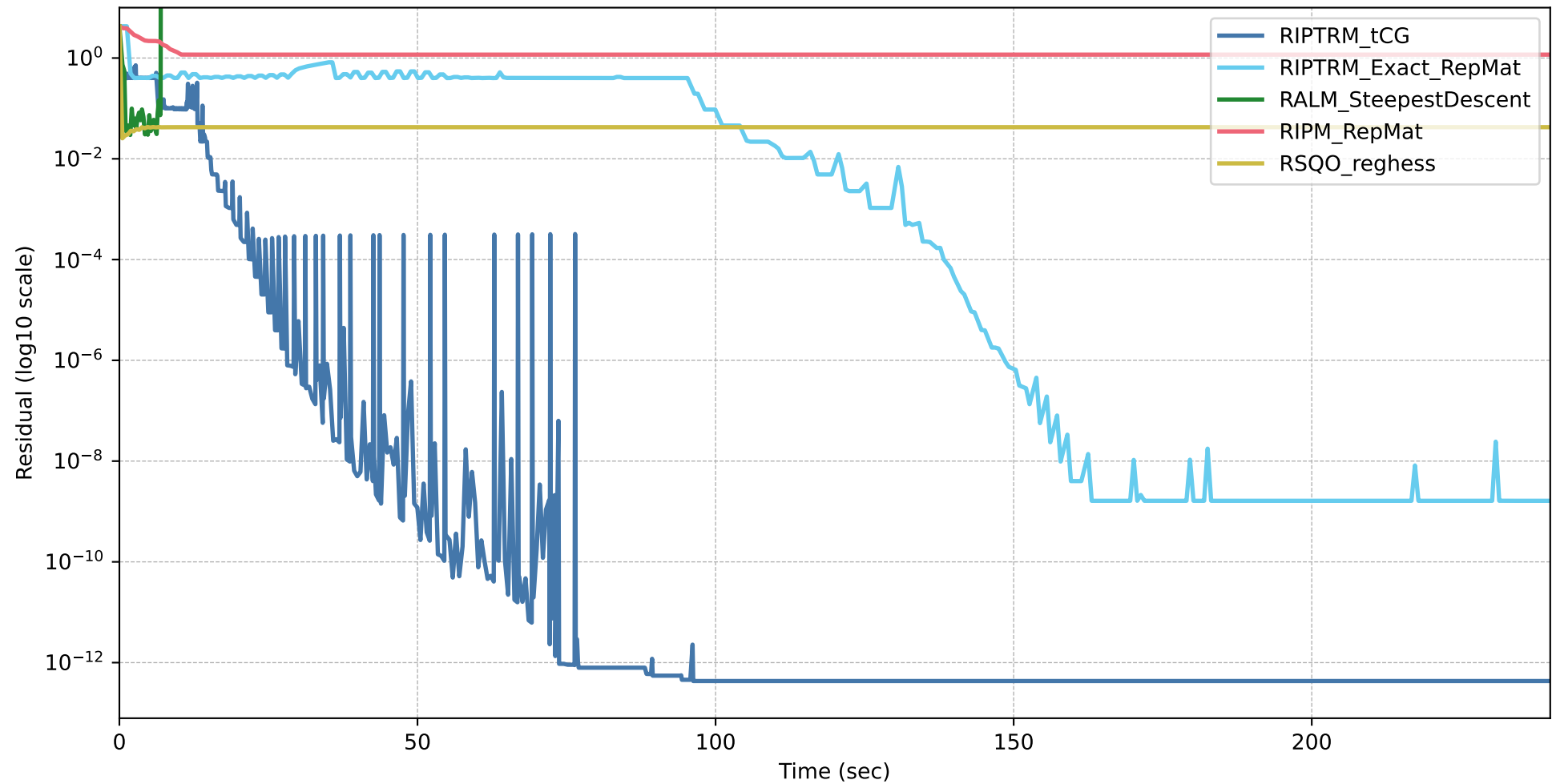
time vs residual for StableIdentification-1-i
