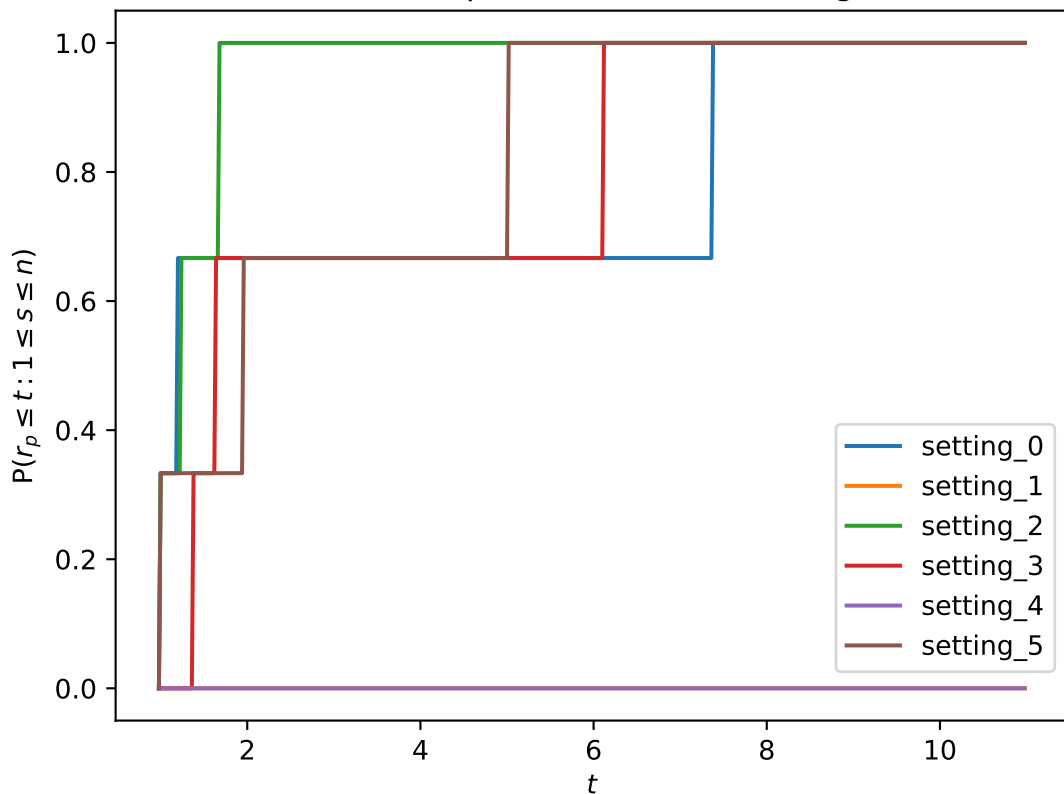
Performance profile (RALM at NonnegPCA)
