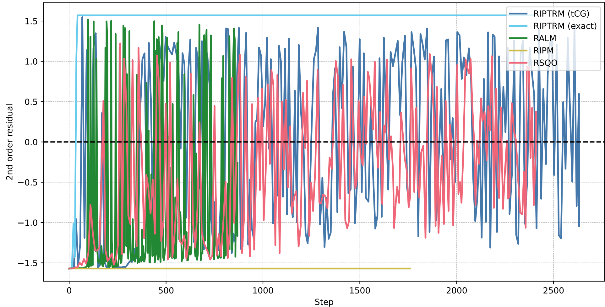
None vs second_order_residual for Rosenbrock-1-a
