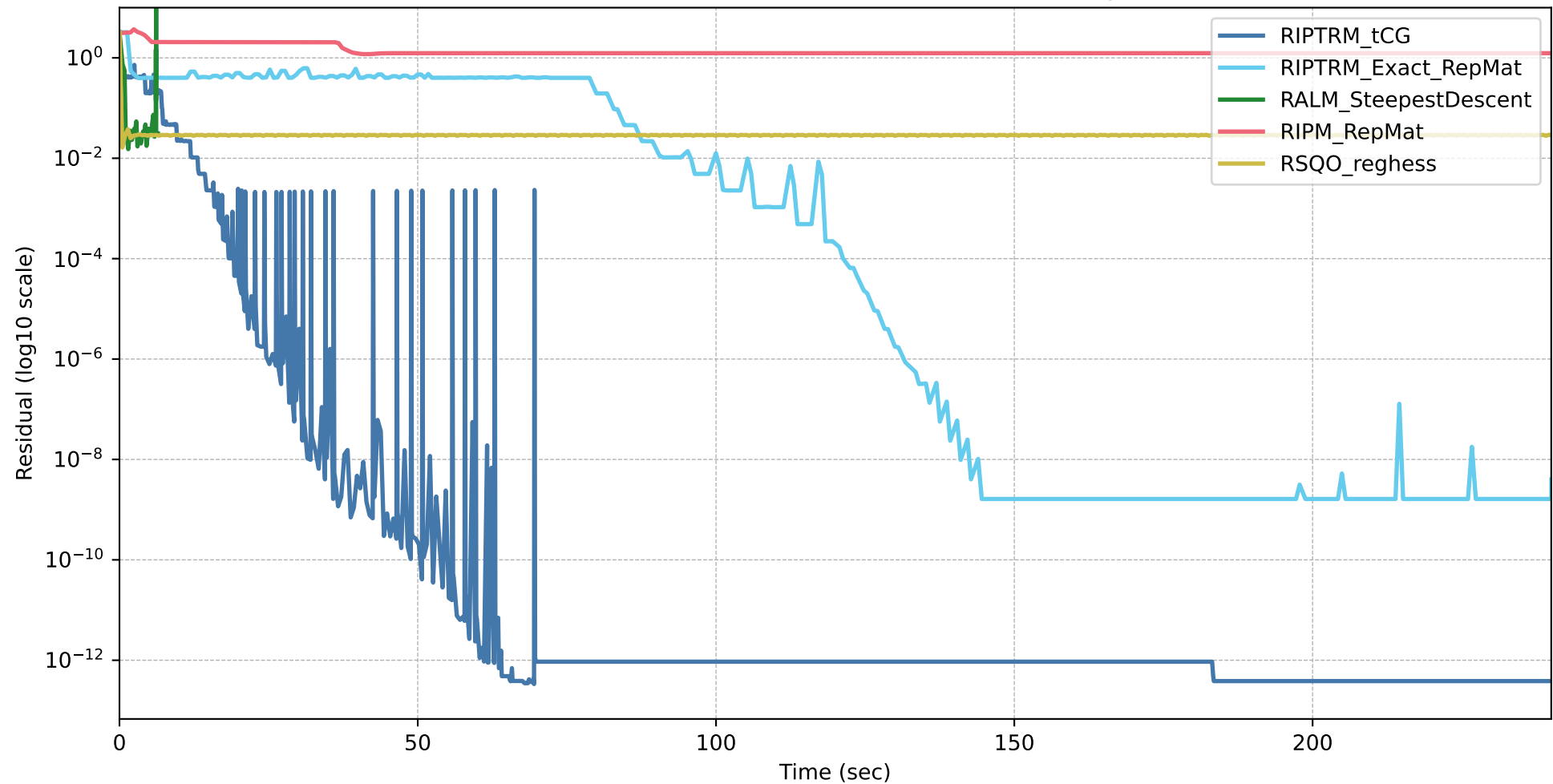
time vs residual for StableIdentification-1-q
