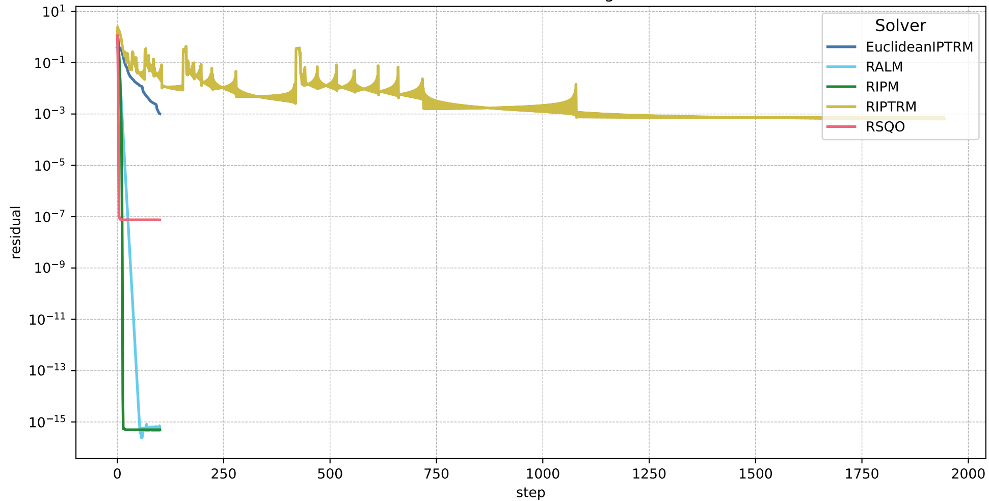
None vs residual for NonnegPCA-1-a
