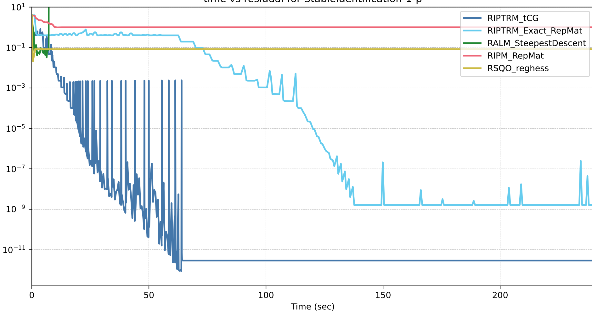
time vs residual for StableIdentification-1-p
