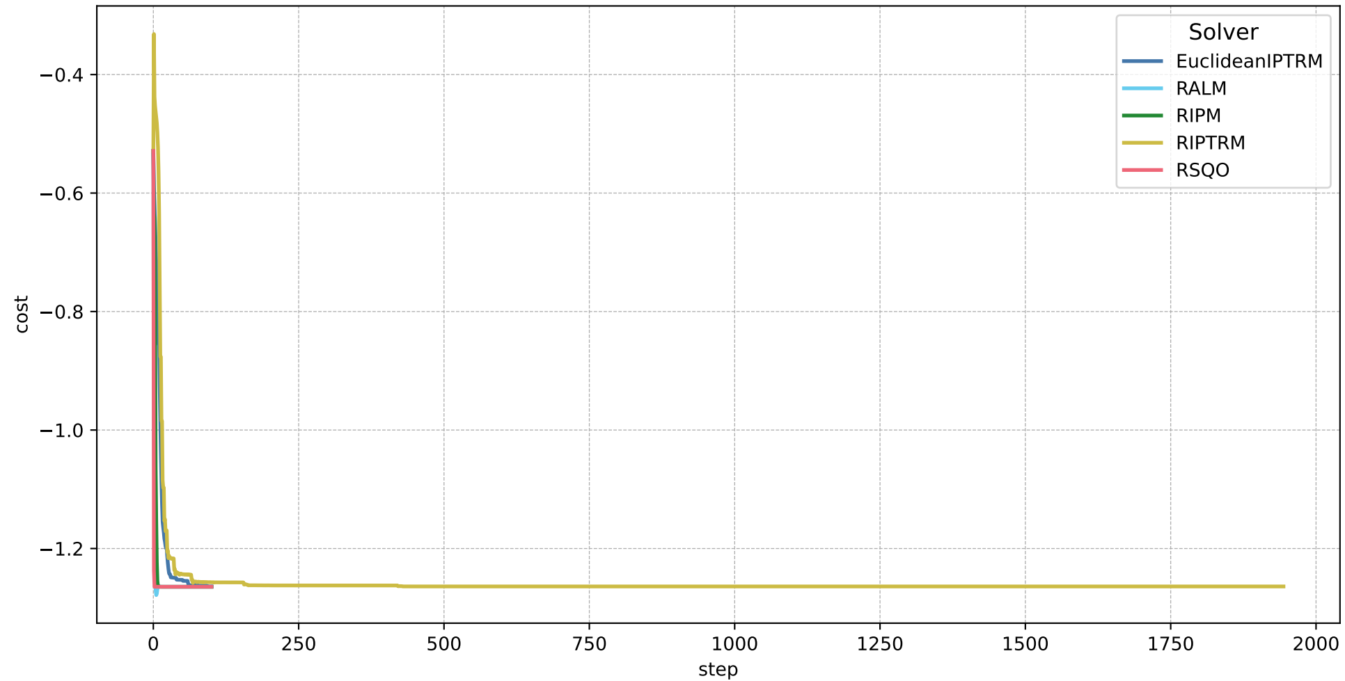
step vs cost for NonnegPCA-1-a
