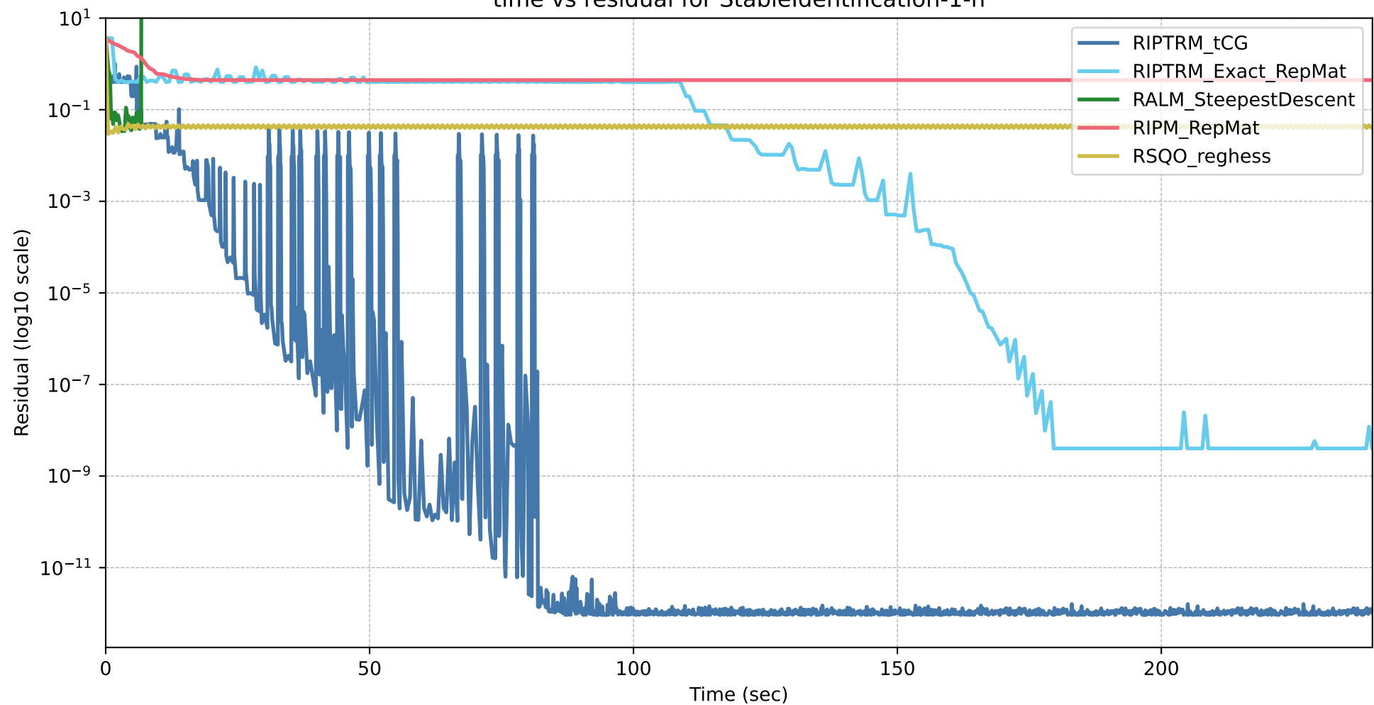
time vs residual for StableIdentification-1-h
