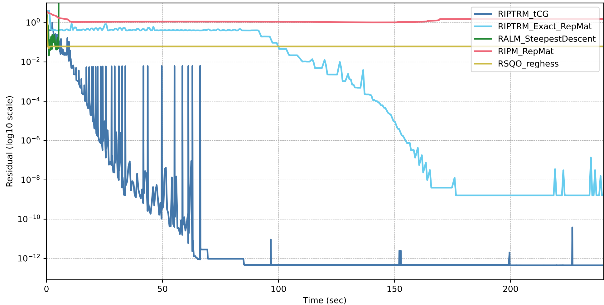
time vs residual for StableIdentification-1-f
