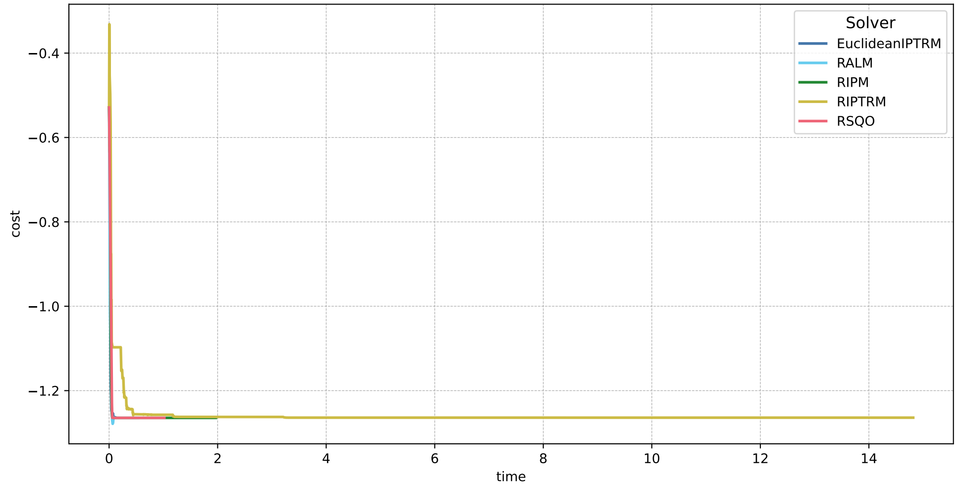
time vs cost for NonnegPCA-1-a
