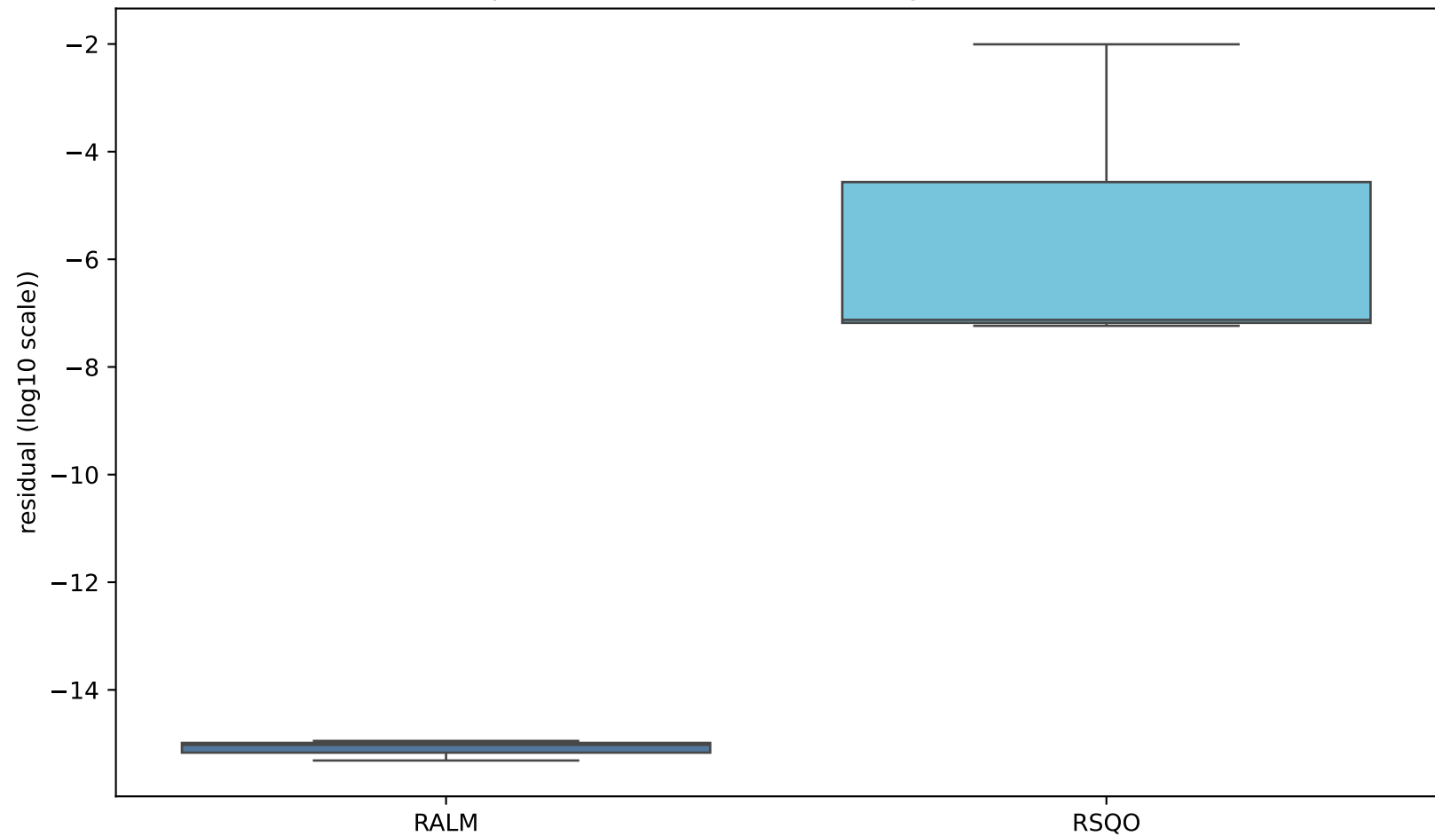
Box plot of residual across NonnegPCA instances
