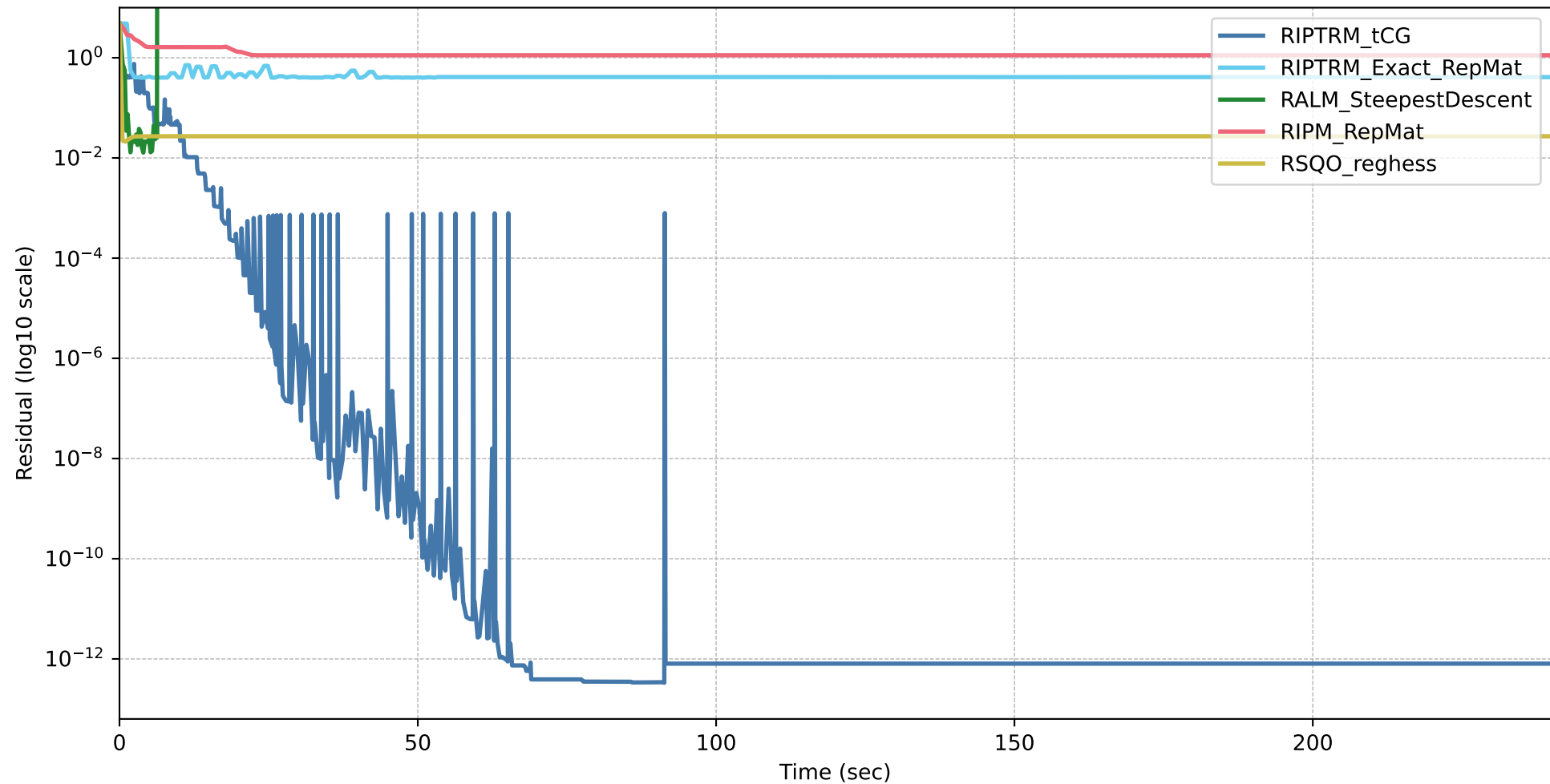
time vs residual for StableIdentification-1-t
