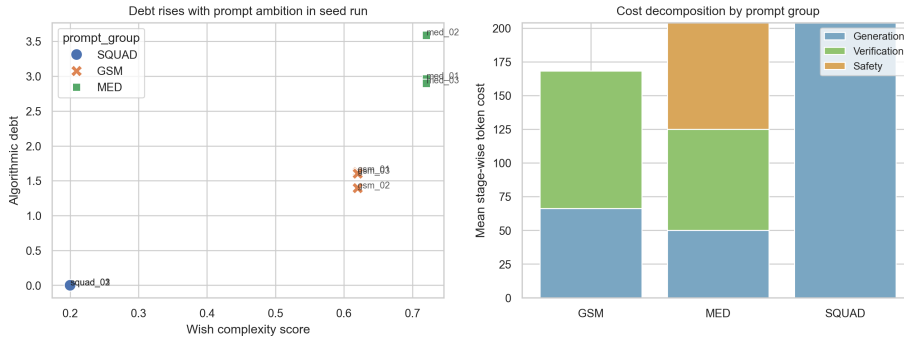
Fig. 3 Measured seed-scale behavior. Left: algorithmic debt against annotated wish complexity. Right: mean stage-wise token cost by prompt group.
