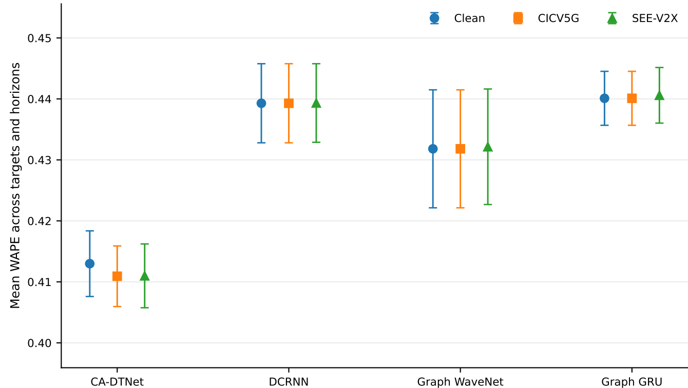
Three-seed forecasting performance under clean and V2X-impaired inputs
