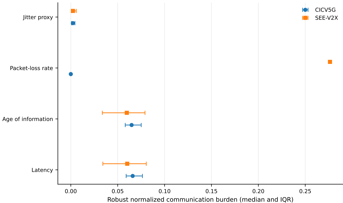
Communication characteristics of the two trace domains
