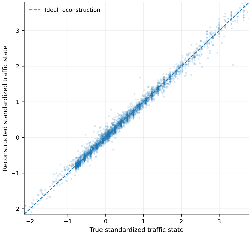
Digital-twin state reconstruction under SEE-V2X ( R^2 = 0.985 )
