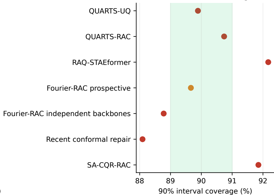
Calibration across stages
