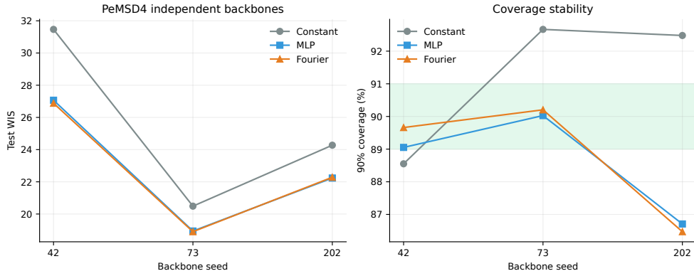
Fig. 6 PeMSD4 WIS and 90% coverage for three independently trained STAEformer backbones. The Fourier advantage reverses for seed 202, and its mean coverage falls below the gate.
