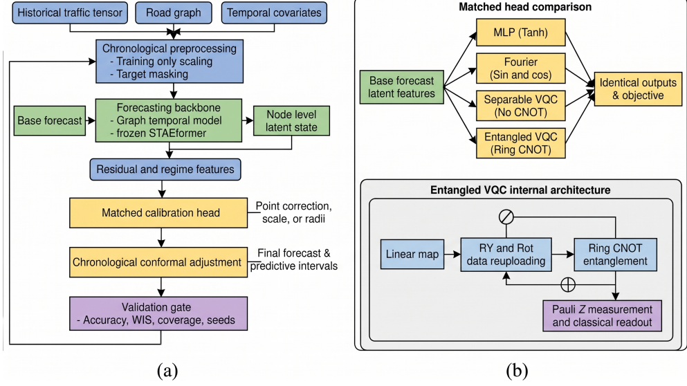
Fig. 1 QUARTS system architecture. Panel (a) shows the chronological data flow through preprocessing, forecasting, residual calibration, conformal adjustment, and validation. Panel (b) shows the matched calibration head comparison and the internal structure of the entangled variational quantum circuit.
