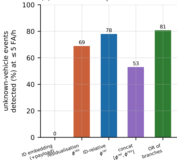
(b) cross-vehicle: representation ablation
