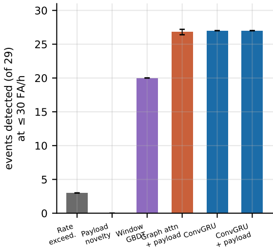
(a) ROAD: detector ablation
