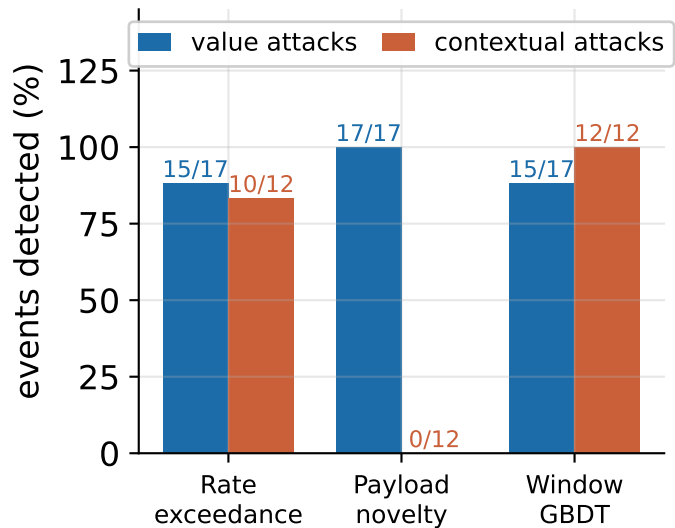
(b) contextual attacks need cross-ID evidence
