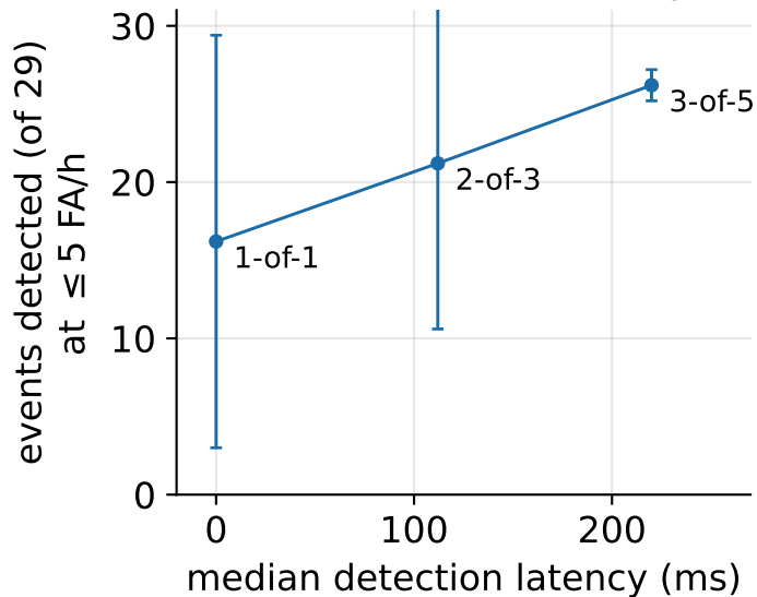
(a) alarm rule sets the latency floor
