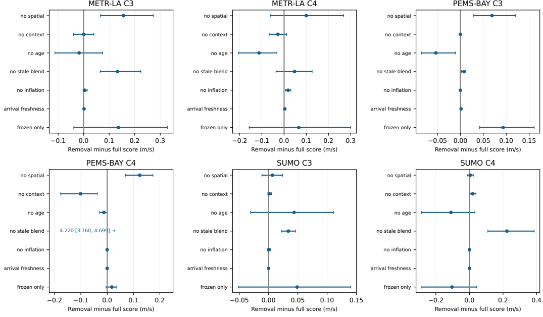
Figure 7. Exploratory removal-minus-full interval-score effects and 95% paired intervals. Positive values indicate deterioration after removal. Panel scales differ; the off-scale PEMS-BAY C4 stale-blend failure is explicitly labelled with its estimate and bounds.
