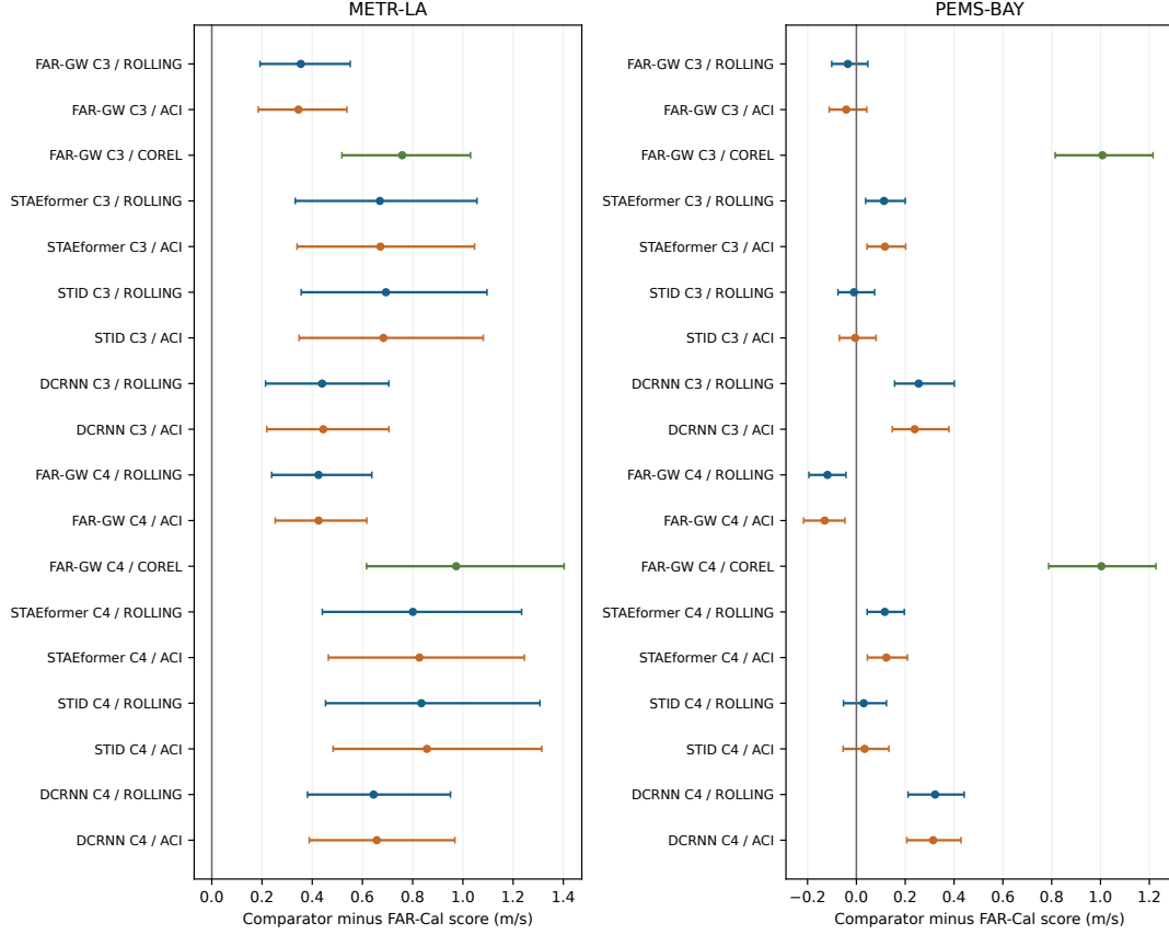
Figure 3. Paired comparator-minus-FAR-Cal interval-score effects and 95% intervals in SI units. Positive values favour FAR-Cal. Comparisons share frozen forecasts within each backbone; CoRel is restricted to FAR-GW.
