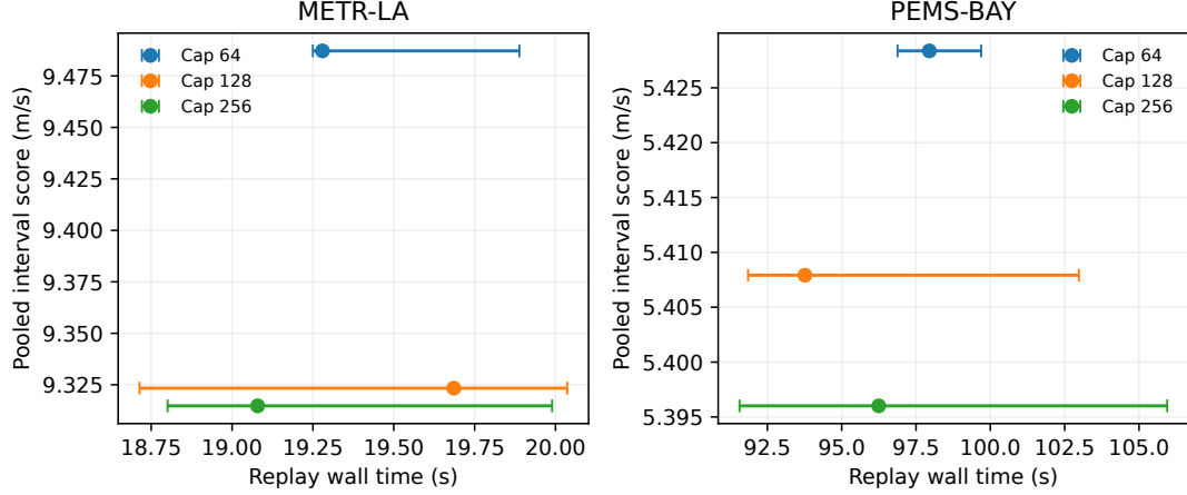
Figure 8. Descriptive archive-cap quality and wall-time sensitivity, with three observed runtime repetitions per cap and network. Horizontal bars are observed ranges, not confidence intervals. These fixed-run pooled scores differ from the origin-level paired inference estimand.
