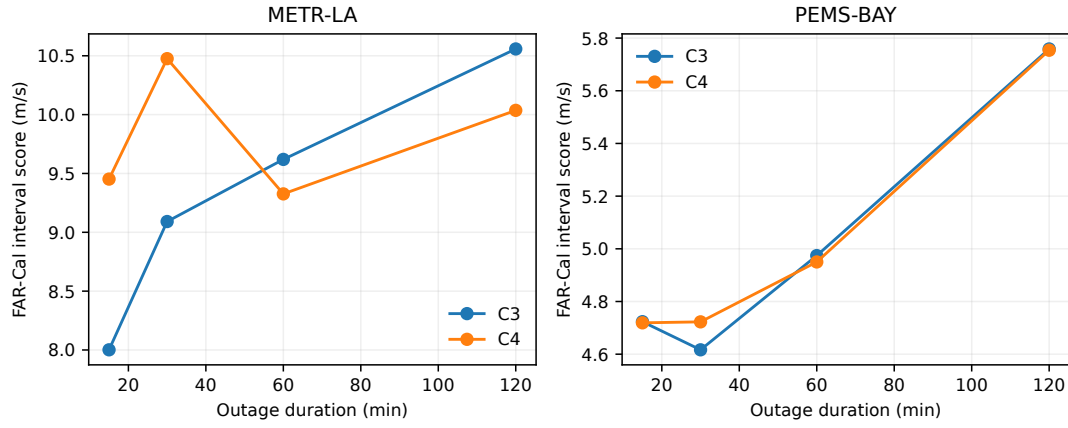
Figure 5. Interval score across the registered outage-duration grid. Lines connect descriptive scores, not interpolation guarantees; C3 and C4 are distinct feedback conditions.
