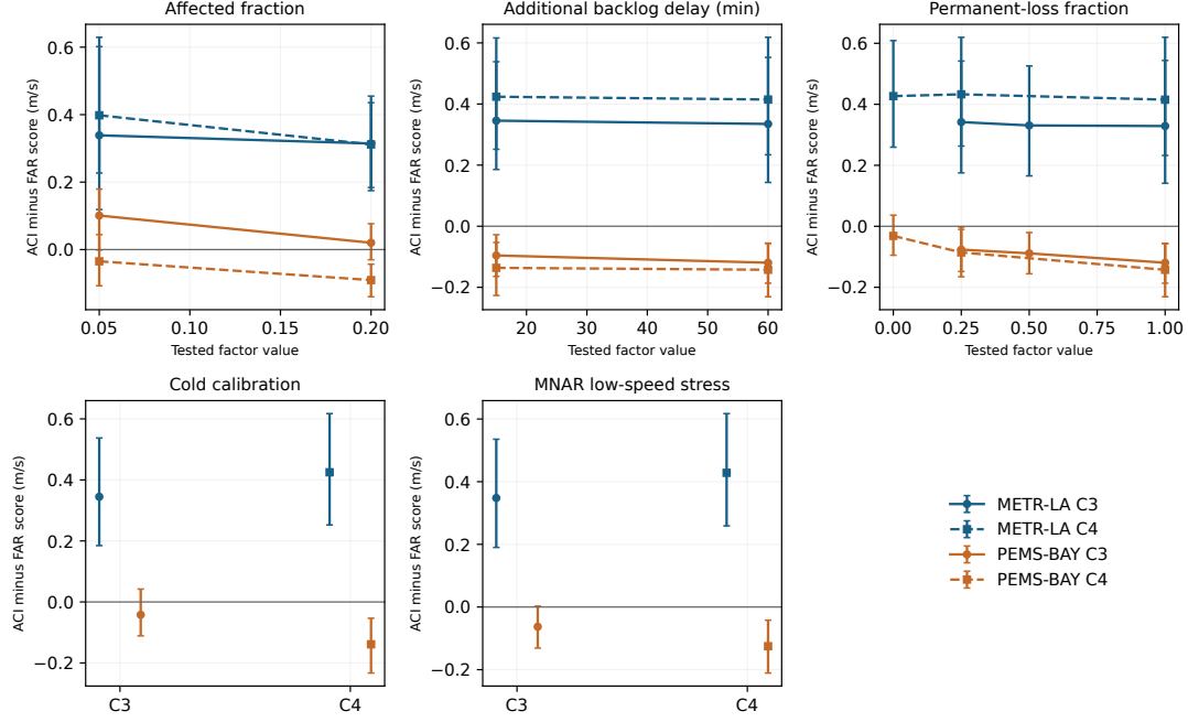
Figure 6. Additional one-factor stress: ACI-minus-FAR-Cal effects and paired 95% intervals for affected fraction, backlog delay, permanent loss, cold calibration and MNAR. Positive values favour FAR-Cal. Categorical panels contain only their registered conditions; continuous lines connect tested values without extrapolation.
