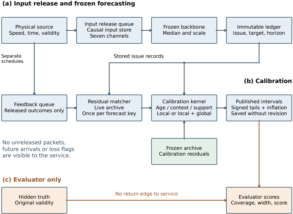
Figure 2. Causal architecture with separate input, feedback and evaluator lanes. Stored issue records feed both residual matching and the calibration query; the junction is intentional. Hidden truth feeds scoring only. All module routes avoid text and preserve the service information boundary.
