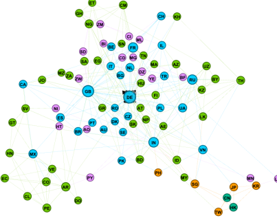
(c) K-means clustering (7 clusters) on node2vec embeddings emphasizing structural equivalence (p=0.25, q=4)
