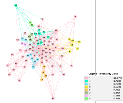
(a) Nodes including the U.S., colored by modularity class
