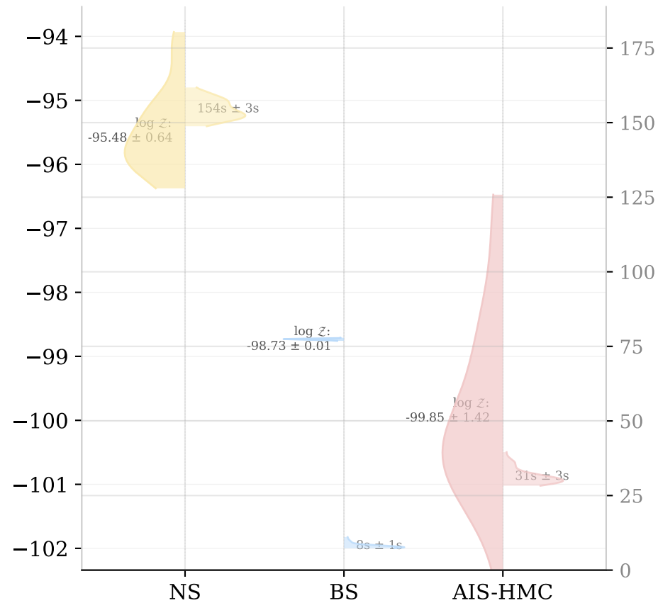
CreditCard (d=29)
