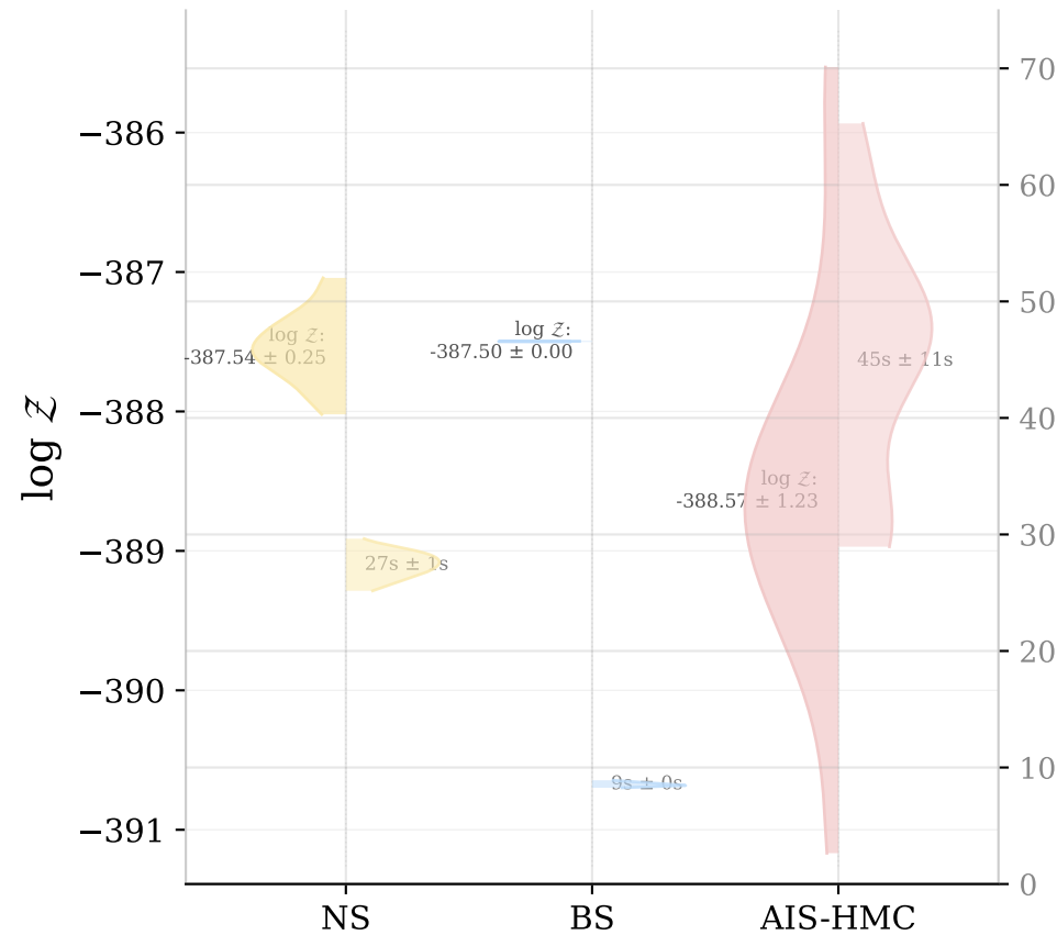
Pima (d=9)
