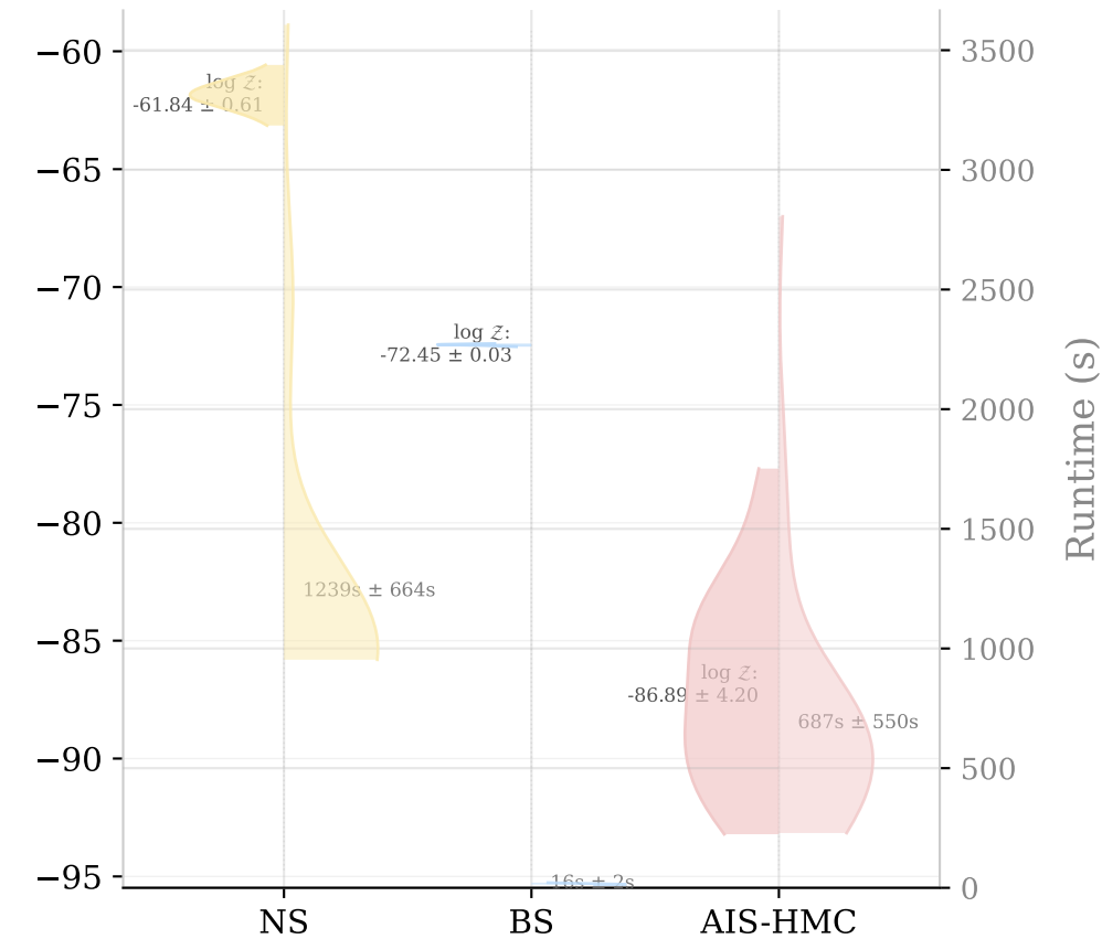
TCGA (d=61)
