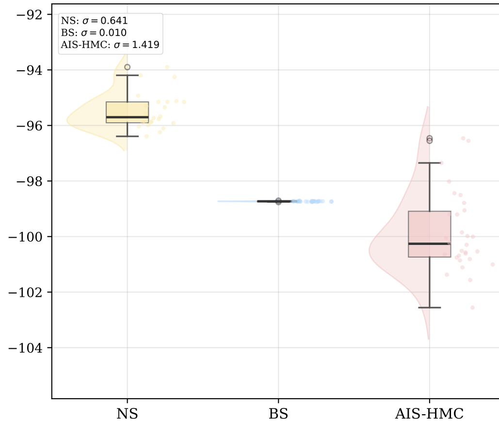
CreditCard (d=29)
