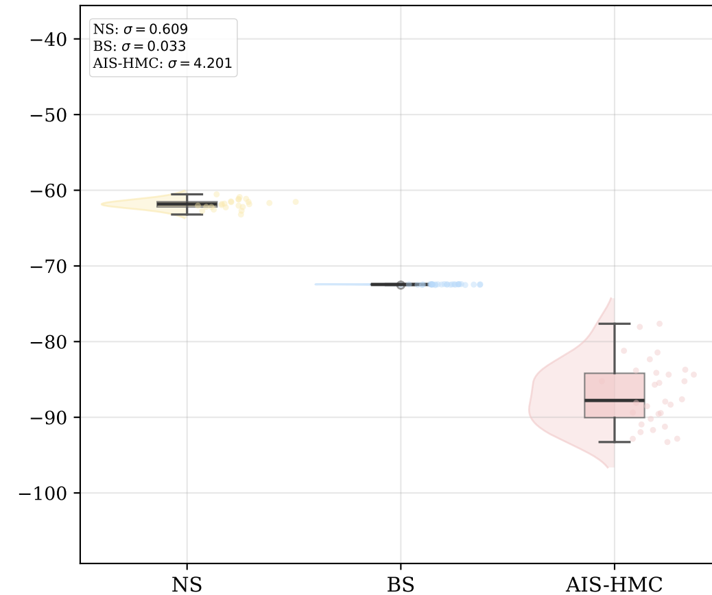
TCGA (d=61)
