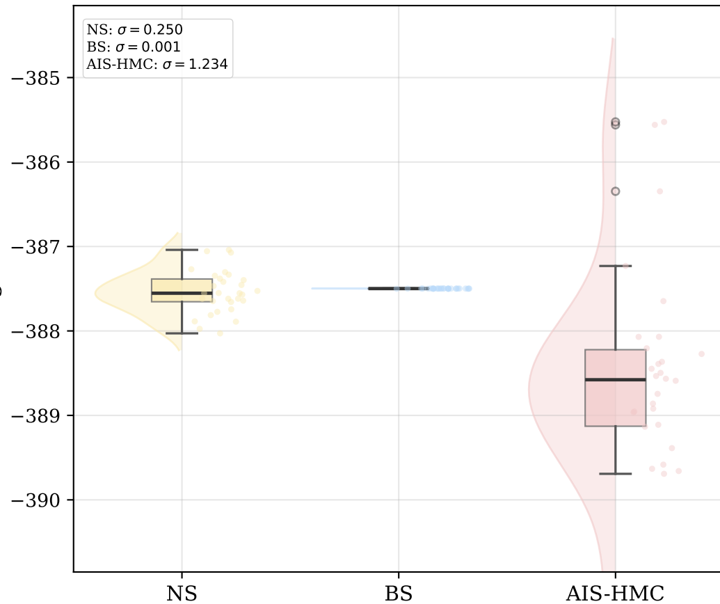
Pima (d=9)
