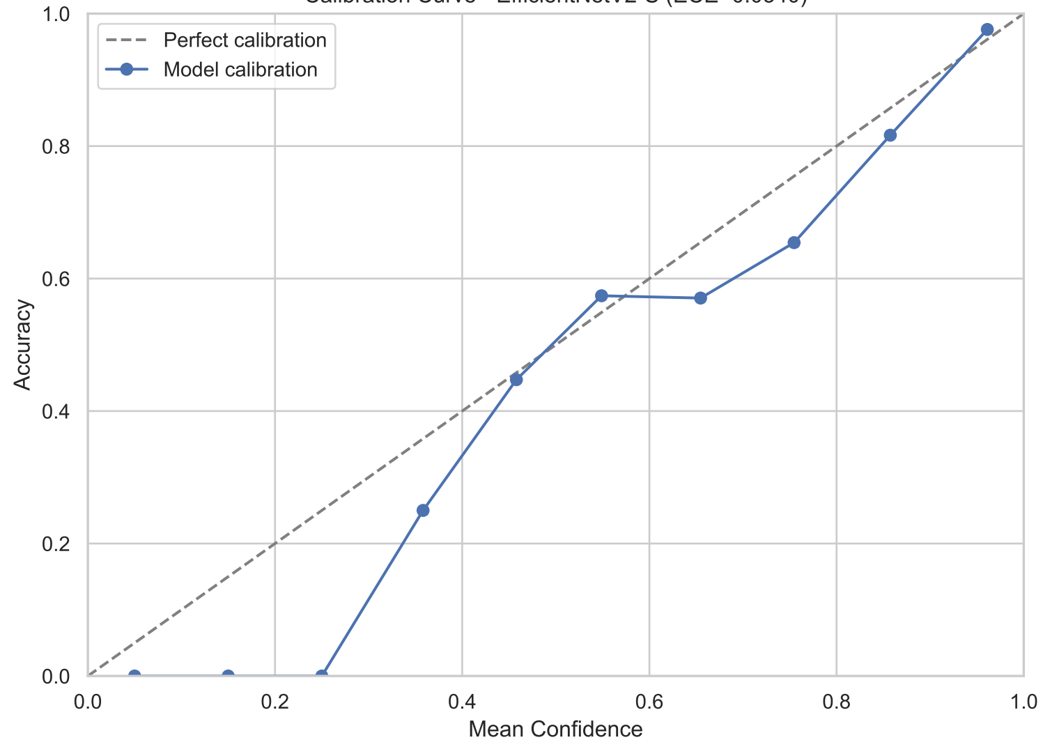
Calibration Curve - EfficientNetV2-S (ECE=0.0340)
