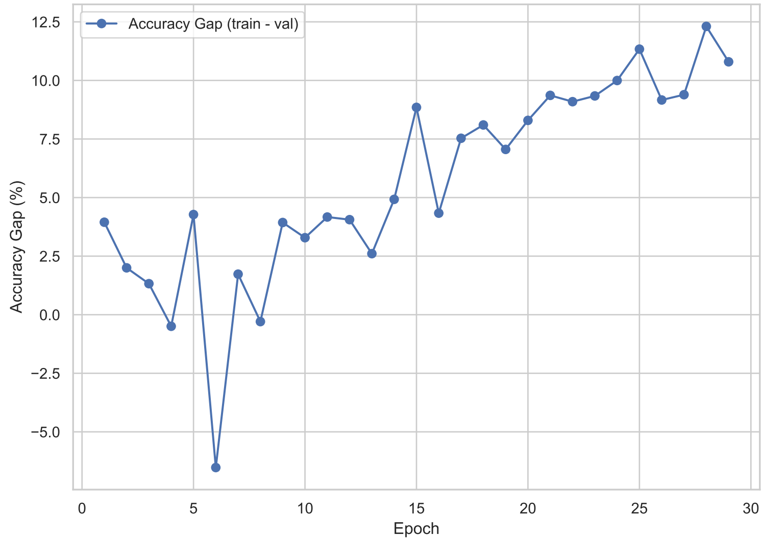
Accuracy Generalization Gap
