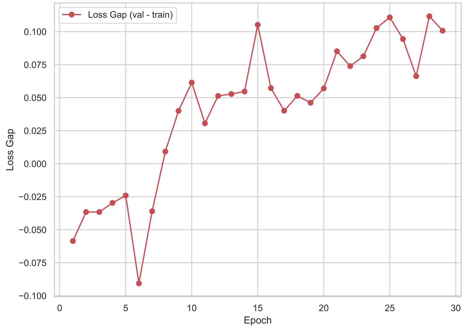
Loss Generalization Gap
