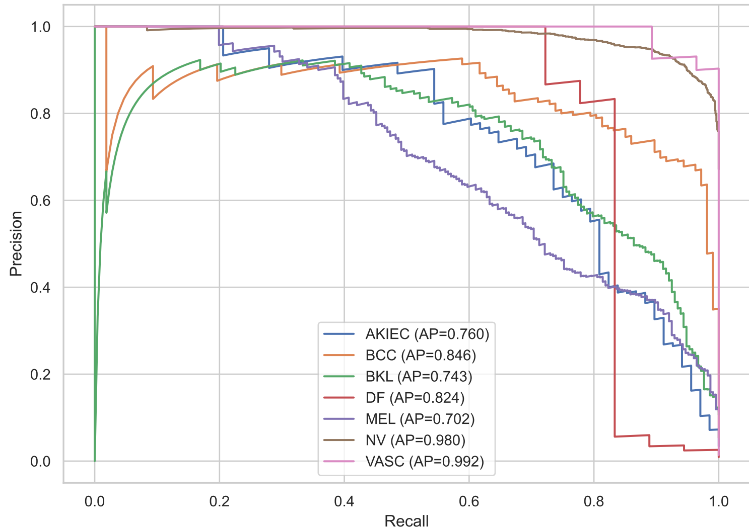
Precision-Recall Curves - EfficientNetV2-S
