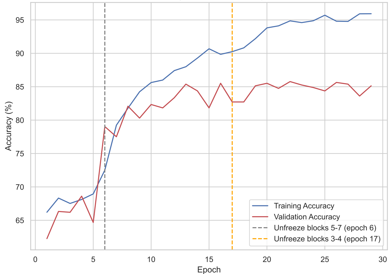
Training & Validation Accuracy
