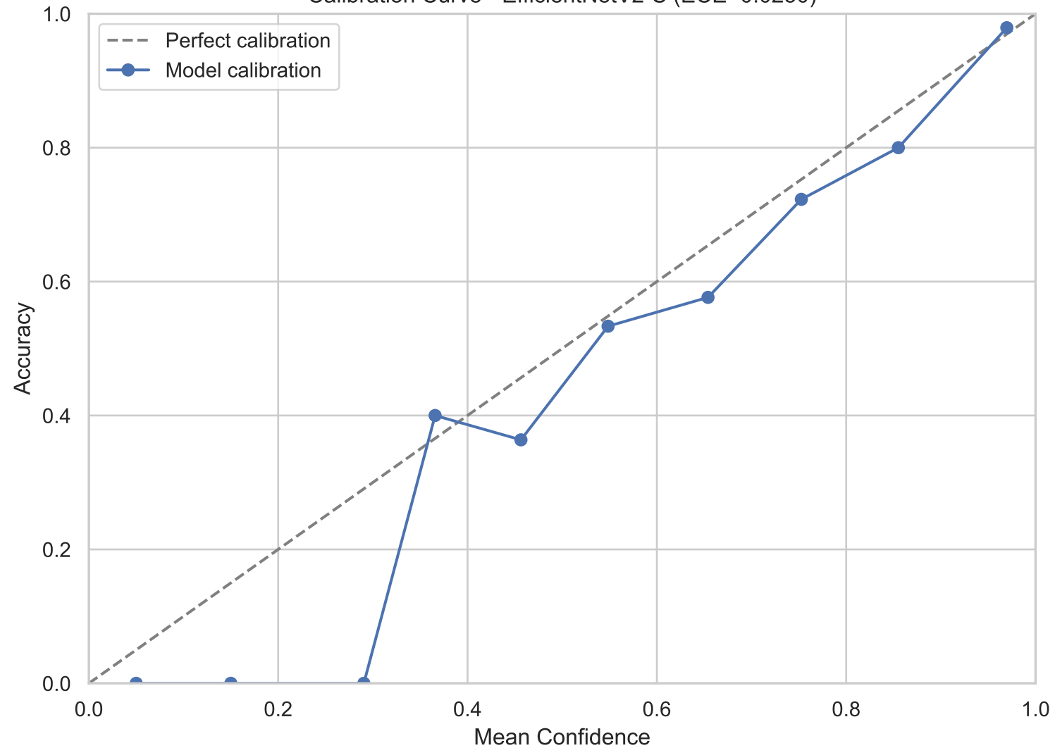
Calibration Curve - EfficientNetV2-S (ECE=0.0250)
