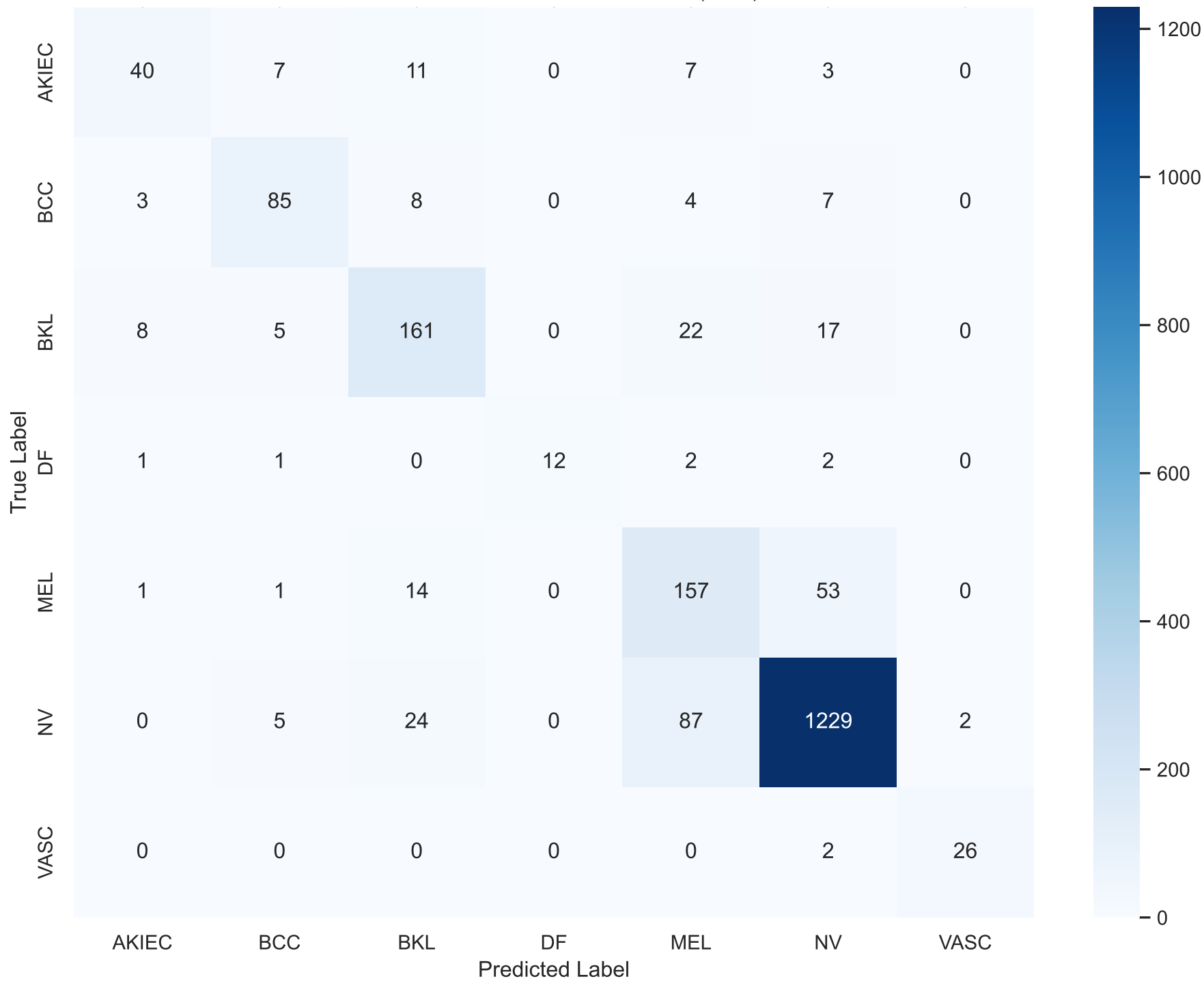
Confusion Matrix - EfficientNetV2-S (Final)
