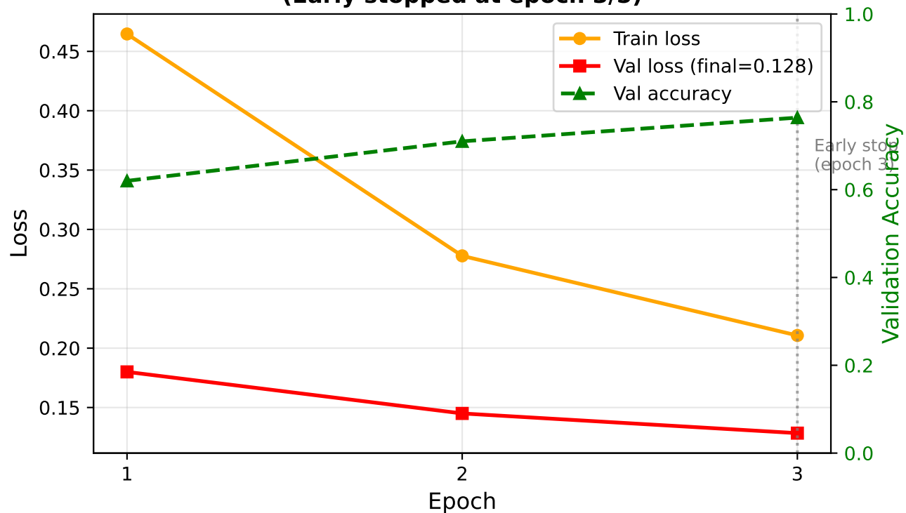
Phase 2 — Supervised Fine-tuning (Early stopped at epoch 3/5)
