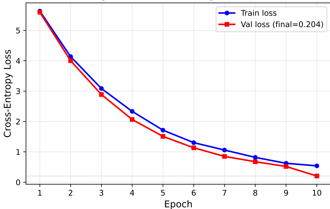
Phase 1 — Causal LM Pre-training (Benign Grammar Learning, 344K flows)
