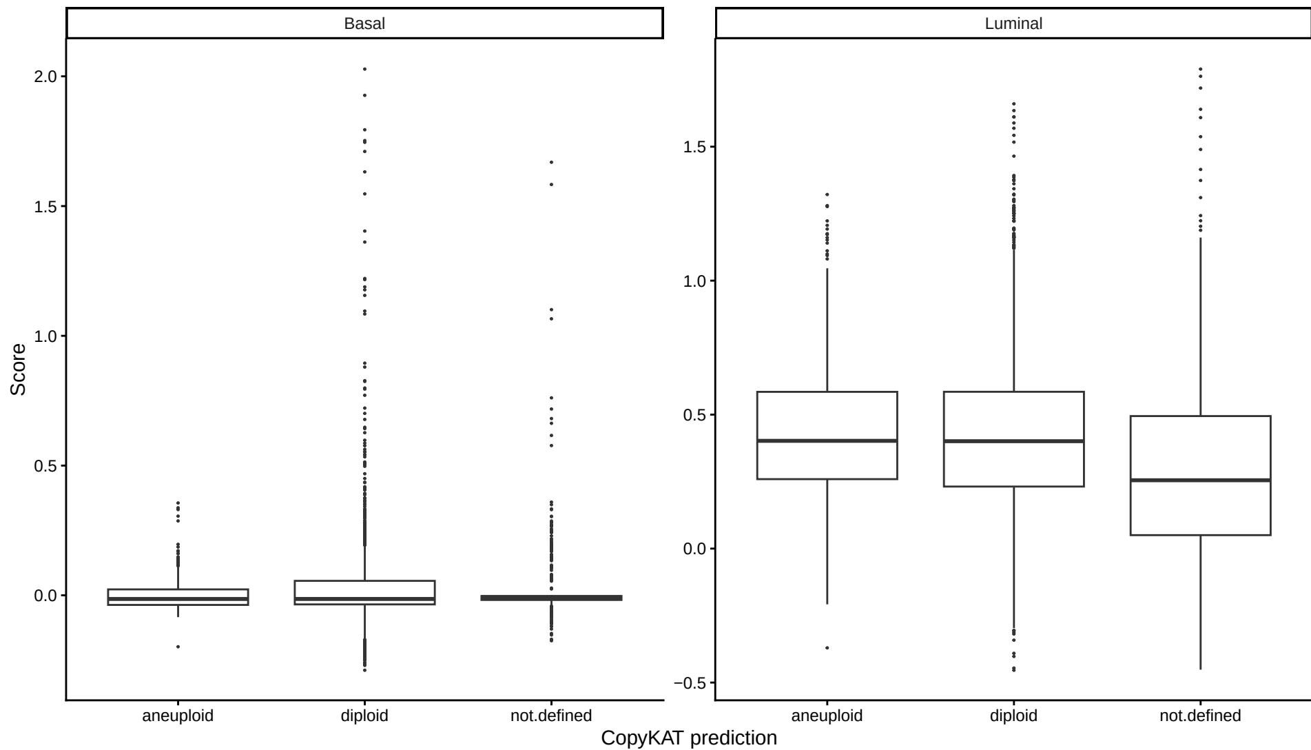
Luminal and Basal Marker Scores by CopyKAT
