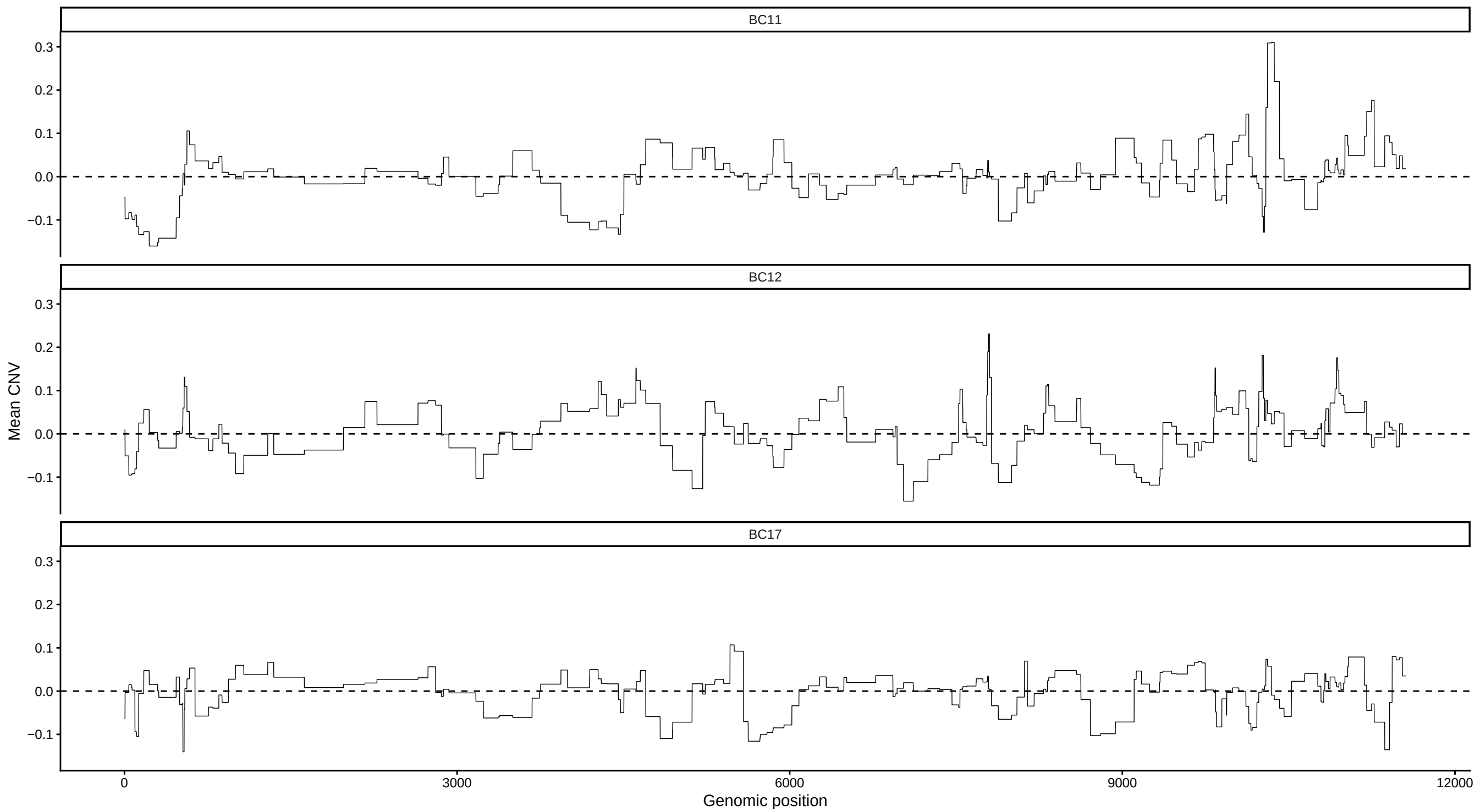
Sample-Specific CNV Profiles in Aneuploid Cells
