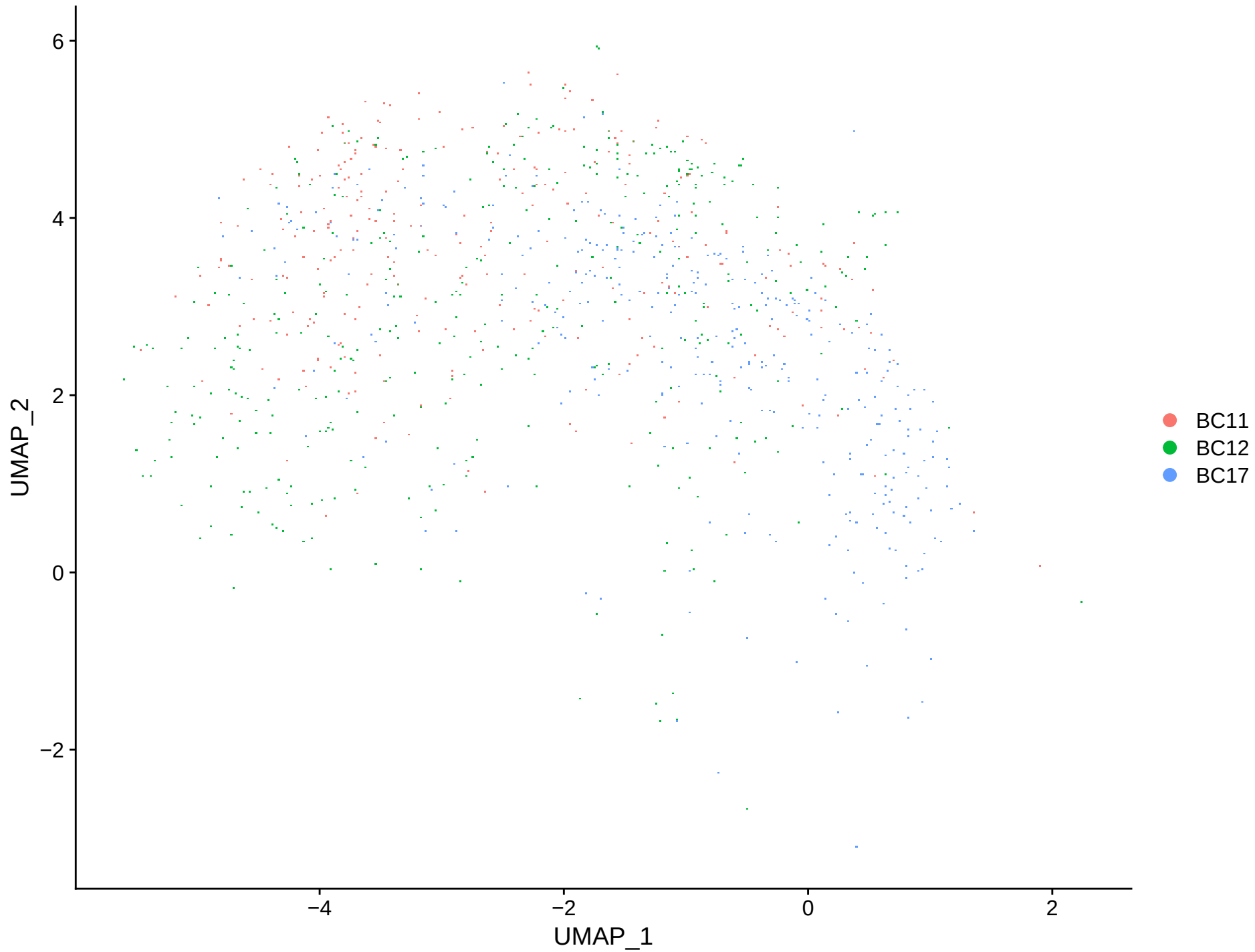
CNV-Supported Malignant Candidates by Sample
