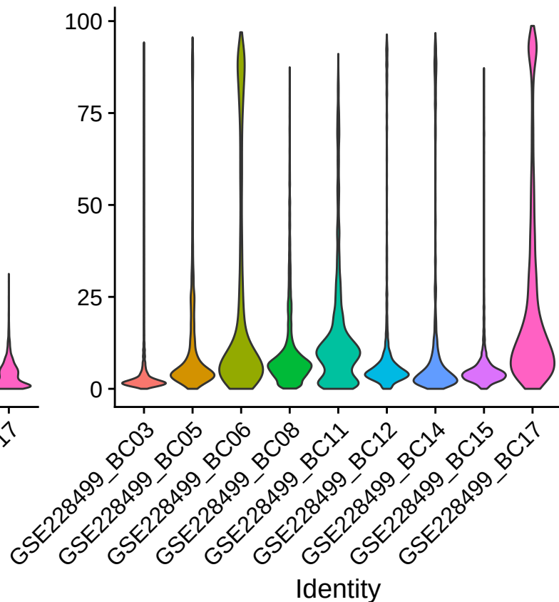
percent.mt
