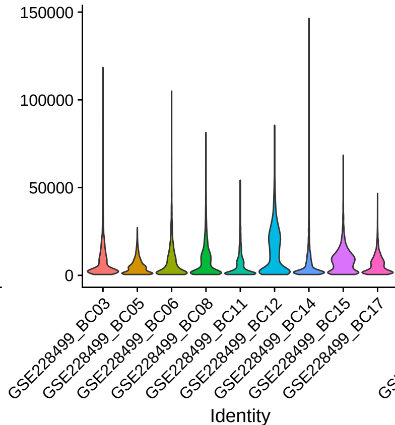
nCount_RNA
