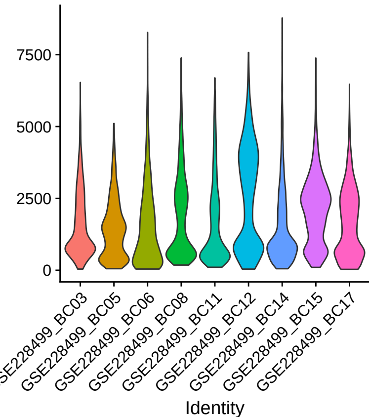
nFeature_RNA
