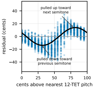
(a) folded residual, EnCodec 3 kbps
