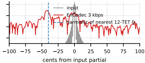
(b) partial 3, 440 Hz, \delta = +40 c
