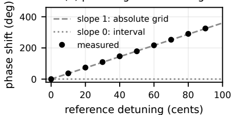
(b) phase against detuning
