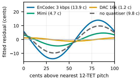
(c) real music: per-bin median, clip-level 95% CI
