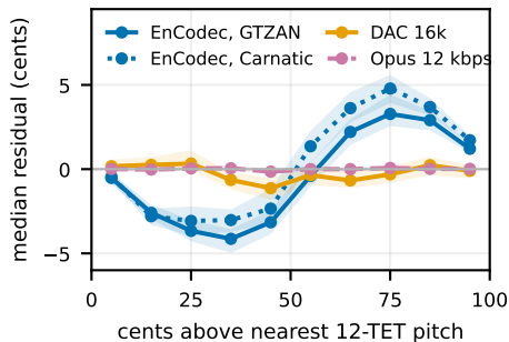
(c) real music: per-bin median, clip-level 95% CI
