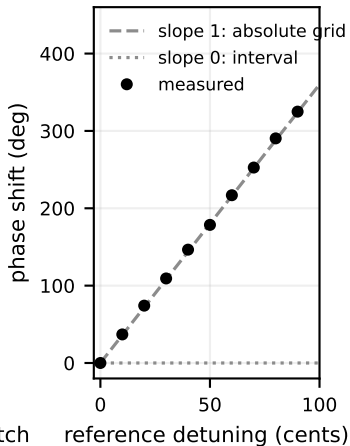
(b) phase against detuning
