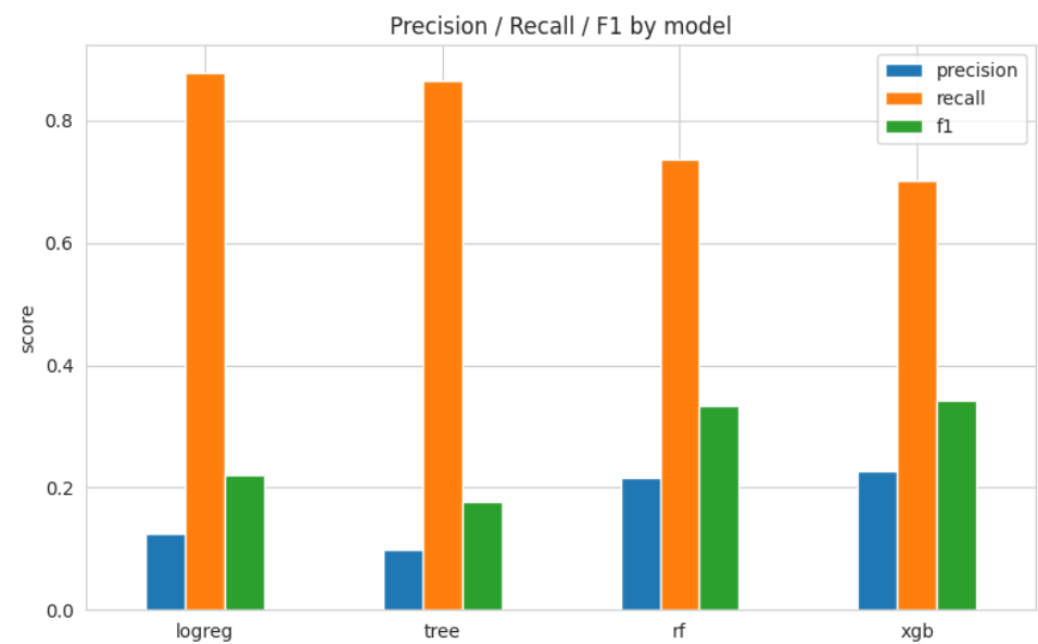
Figure 2. Precision, recall, and F1 across all four models at the default threshold.
