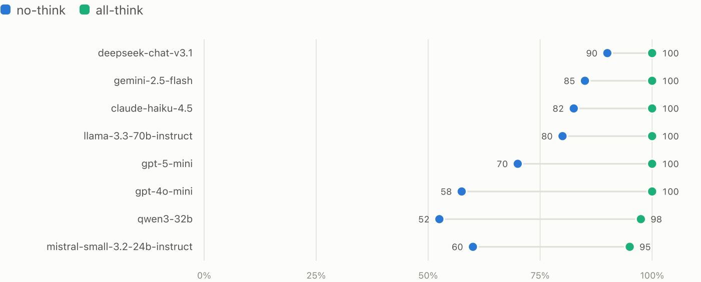
FIGURE 4 Correct rate by model: no-think vs all-think
