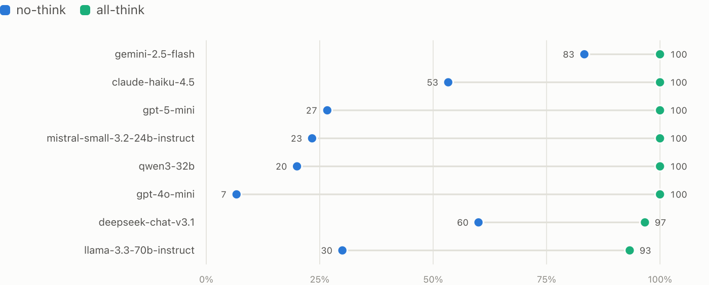
FIGURE 1 Correct rate by model: no-think vs all-think
