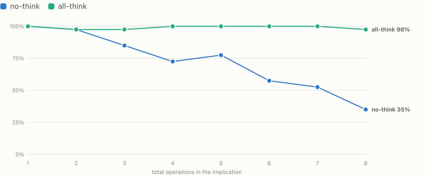
FIGURE 5 Accuracy vs implication complexity
