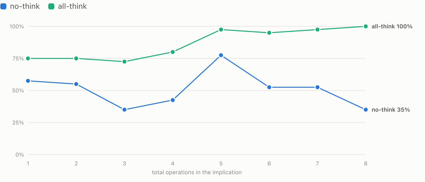
FIGURE 5 Accuracy vs implication complexity
