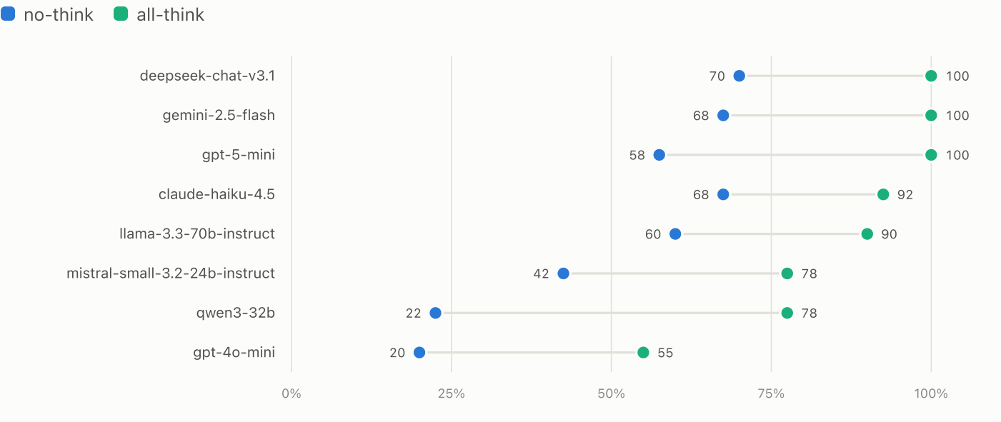
FIGURE 4 Correct rate by model: no-think vs all-think
