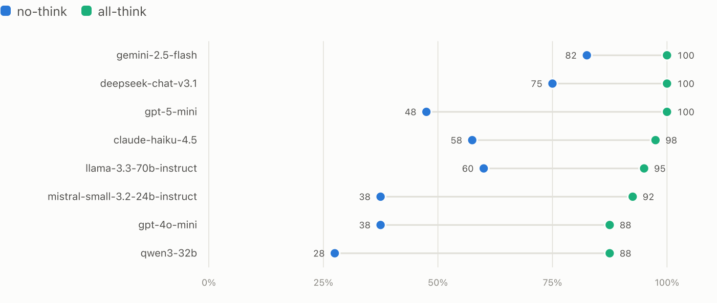
FIGURE 4 Correct rate by model: no-think vs all-think
