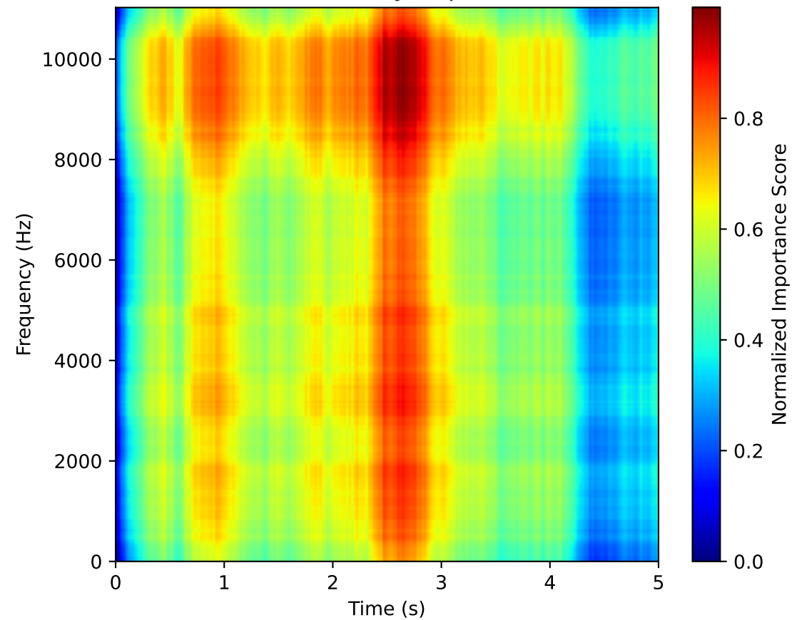
Saliency Map
