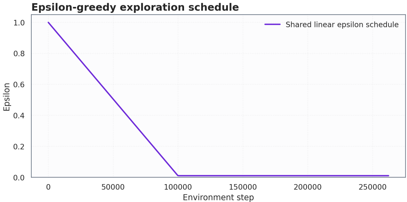
Figure 1: Shared epsilon-greedy schedule
