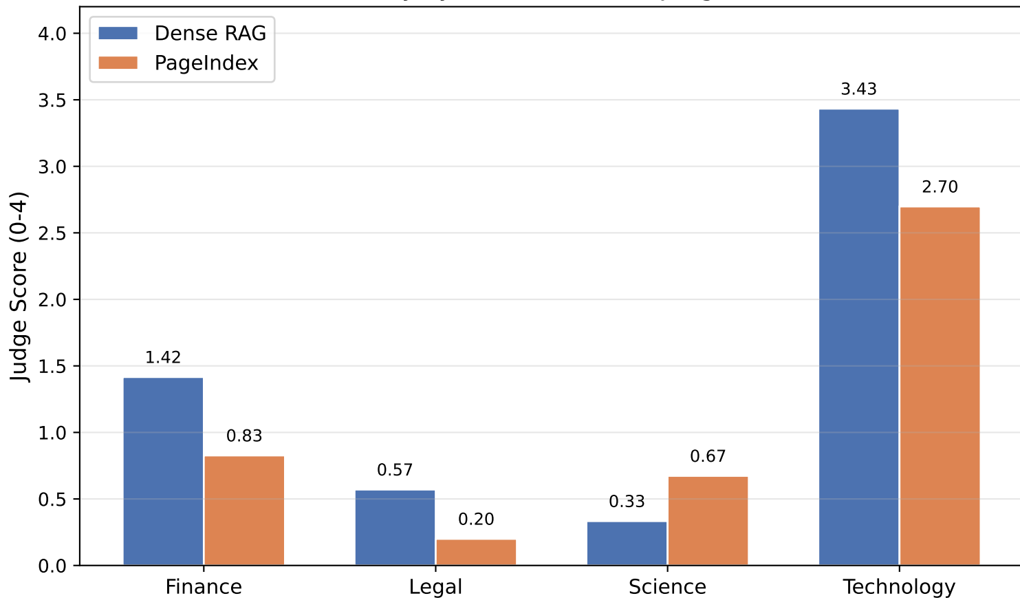
RQ1: Accuracy by Domain (LLM-as-Judge, 0-4 scale)
