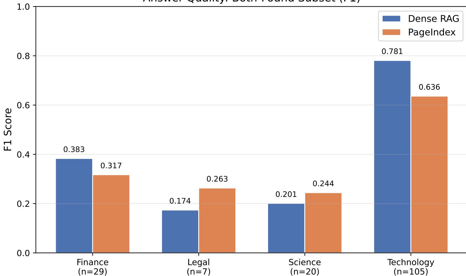
Answer Quality: Both-Found Subset (F1)
