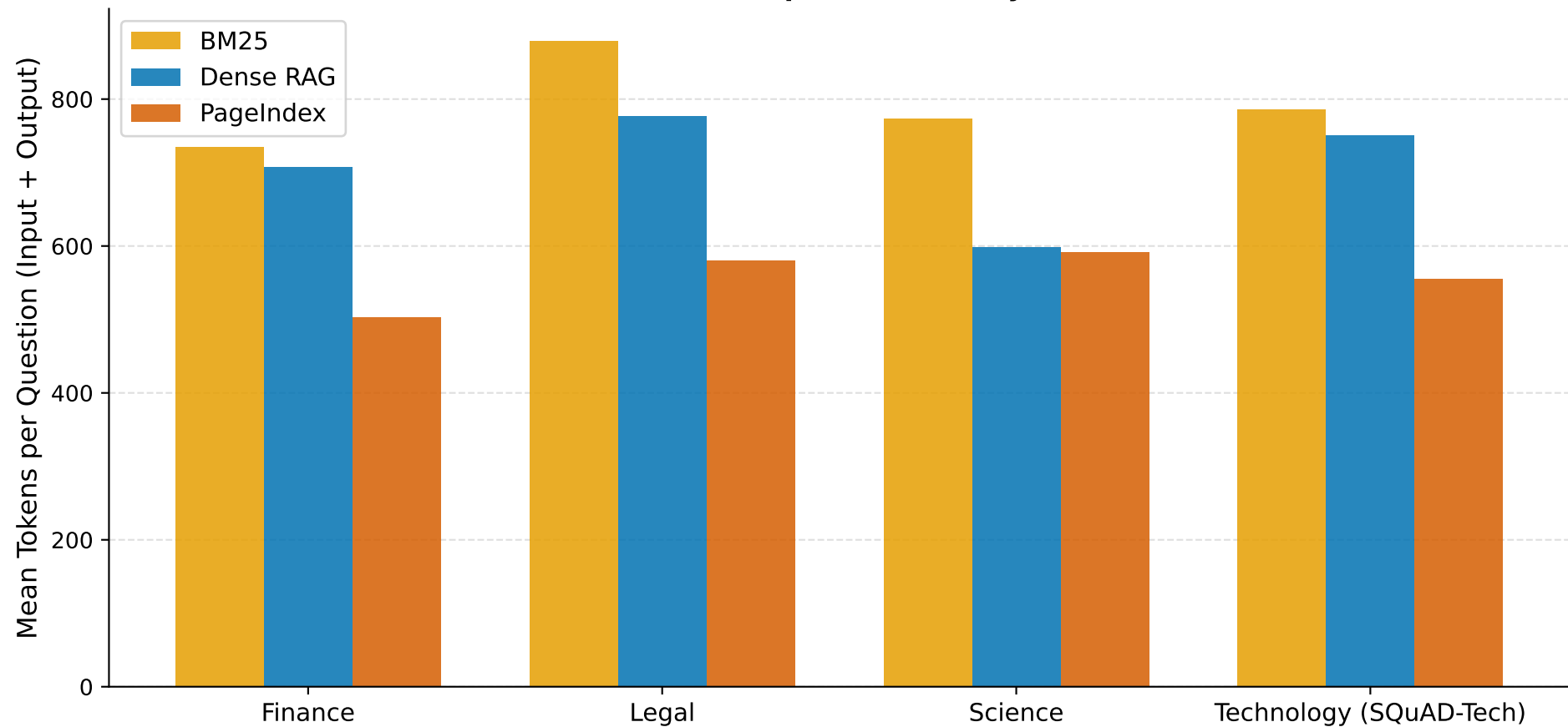
RQ3: Token Cost per Question by Domain
