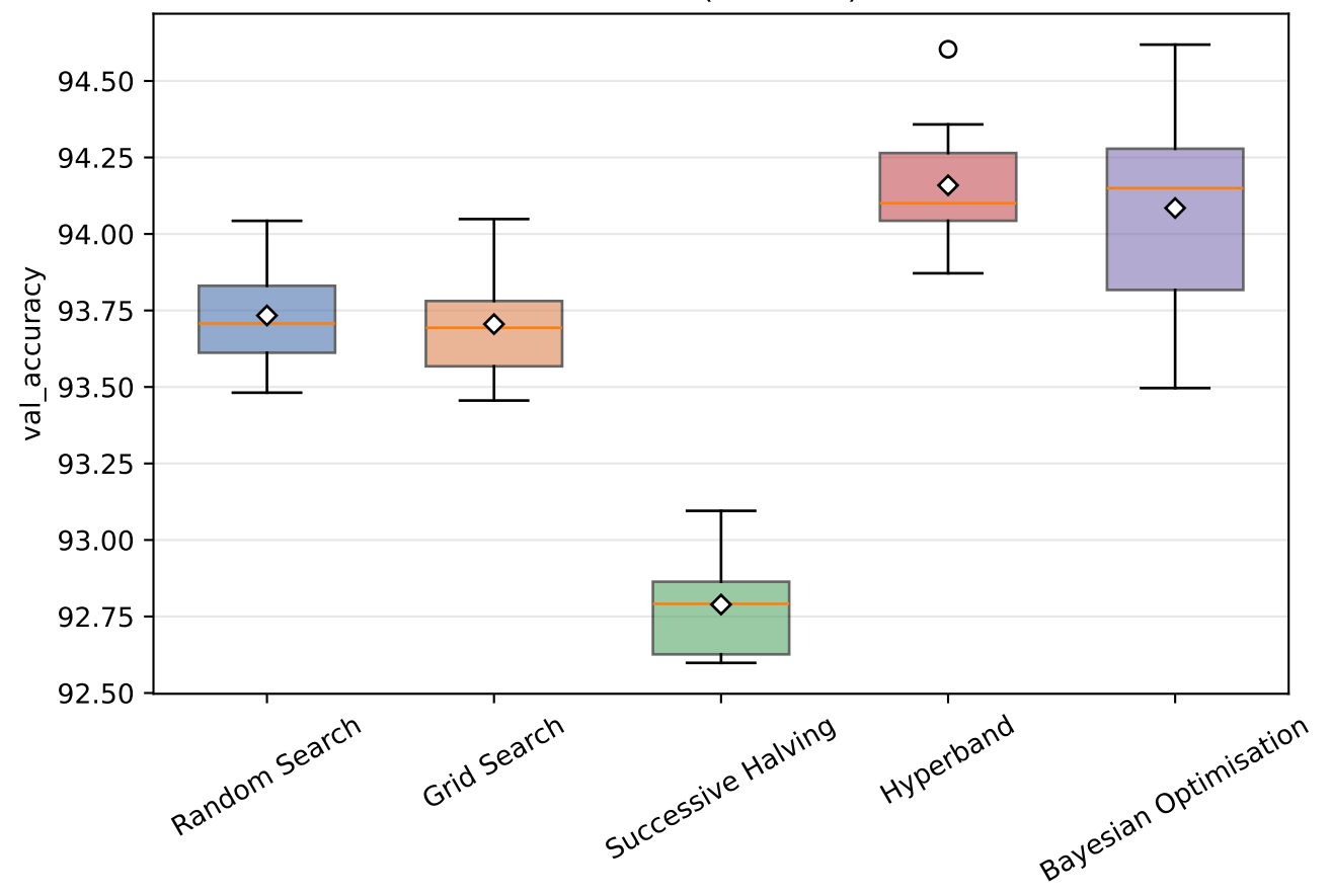
NB301 (CIFAR10)
