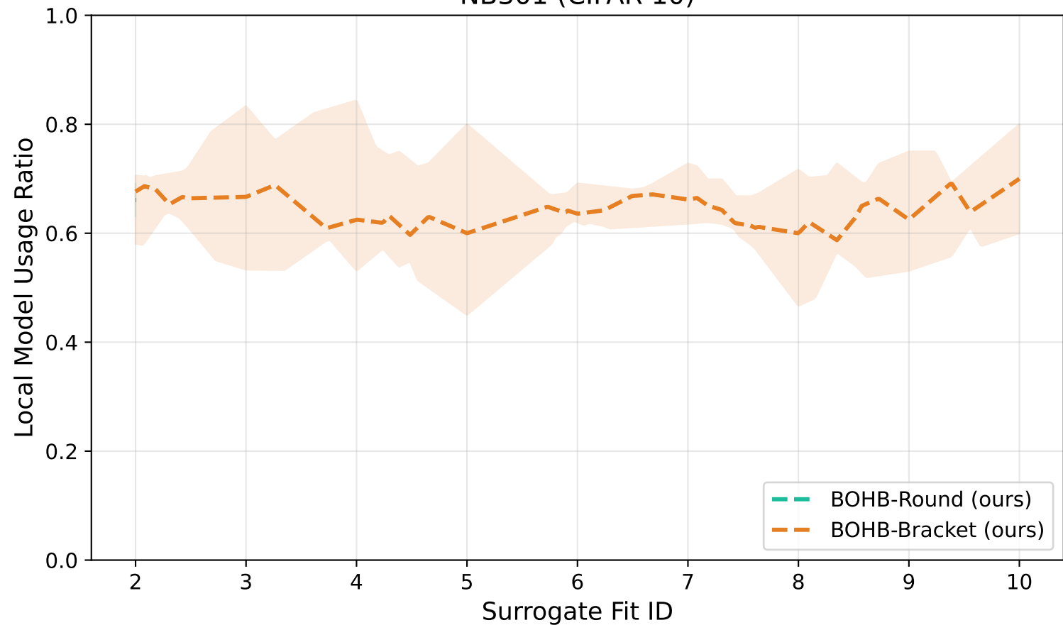
NB301 (CIFAR-10)
