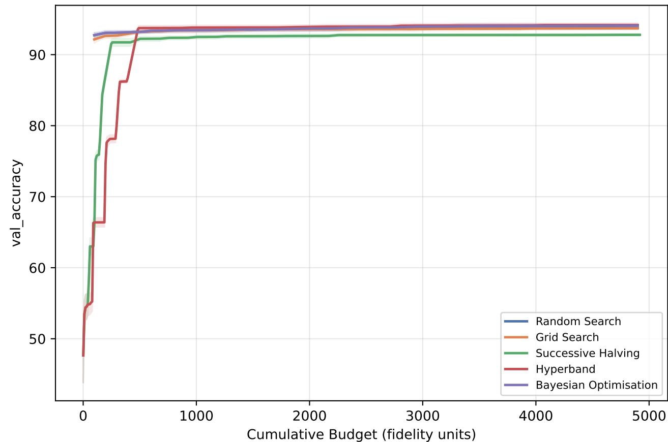
NB301 (CIFAR10)
