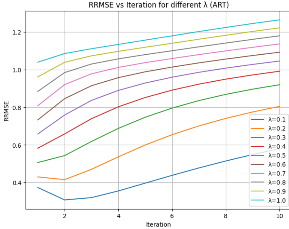
Figure 14: RRMSE as a function of iteration number for different values of step-length \lambda .
