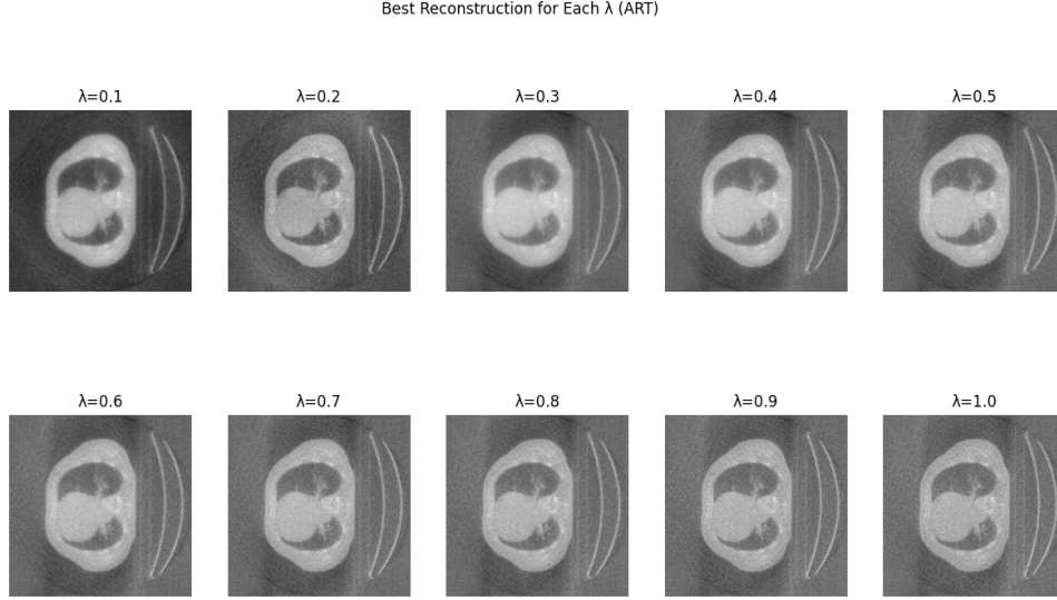
Figure 13: Reconstructed image using ART with noisy projection data.
