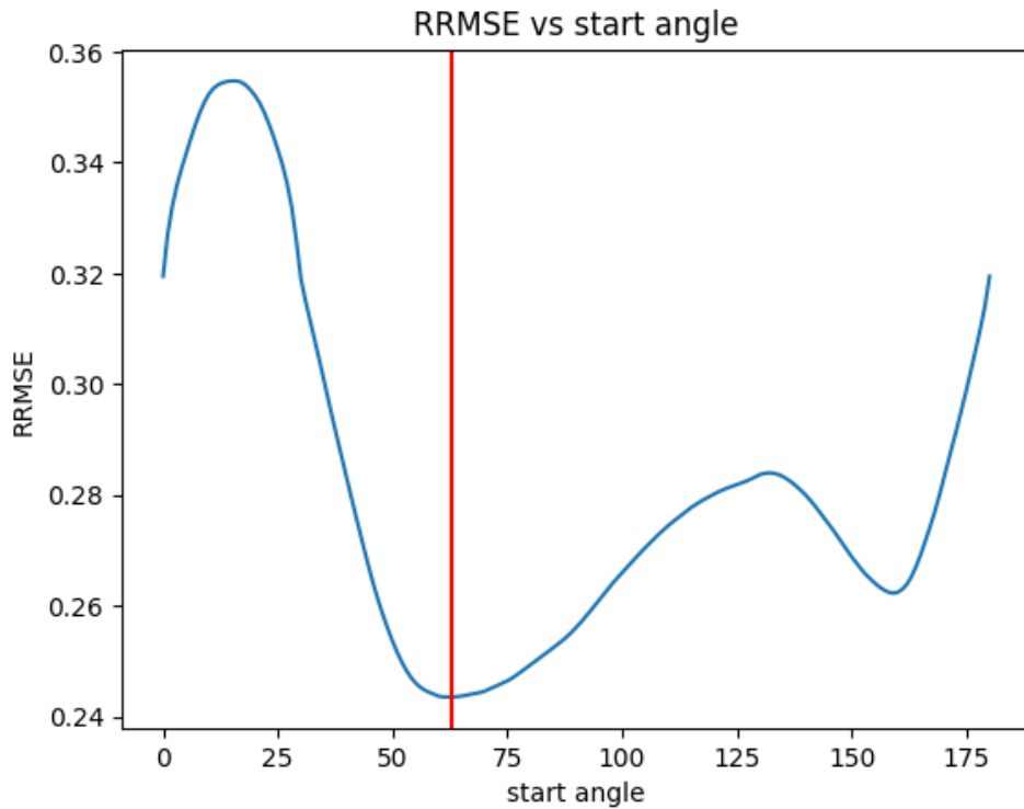
Figure 7: RRMSE as a function of starting angle \theta for the chestCT dataset.
