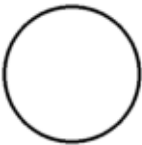
easy #00000014
