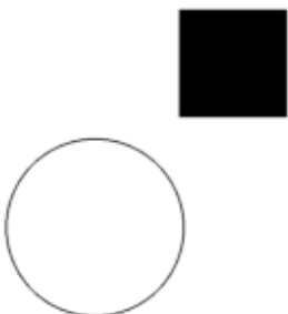
easy #00000008
