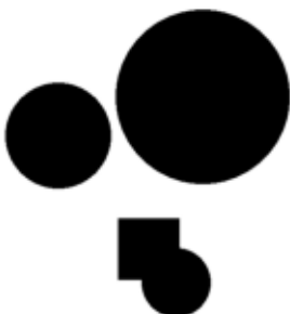
medium #00000039
