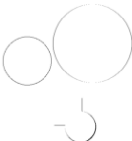
XOR diff
