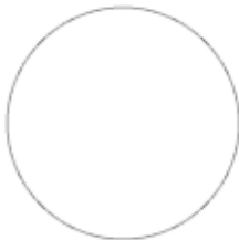
XOR diff
