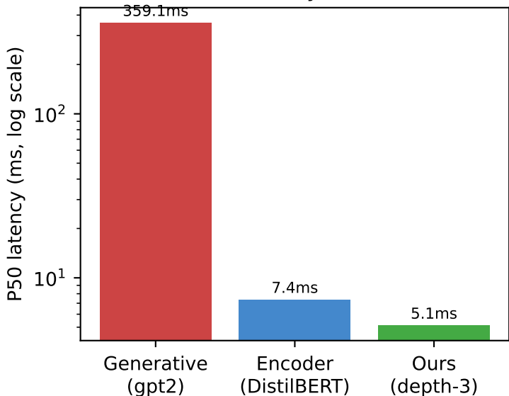
Inference latency on ATIS (C2)
