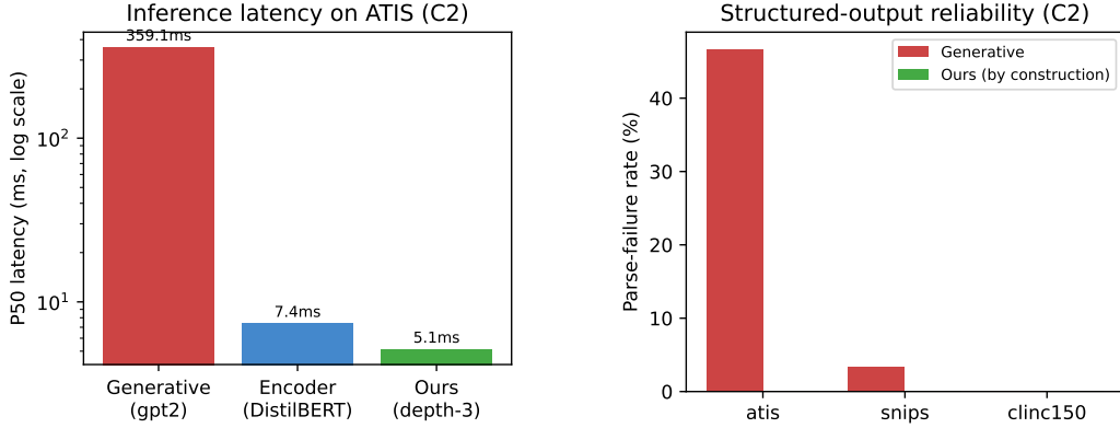
Figure 3: Left: P50 CPU latency on ATIS (log scale). Right: structured-output parse-failure rate; ours is 0% by construction regardless of schema size.
