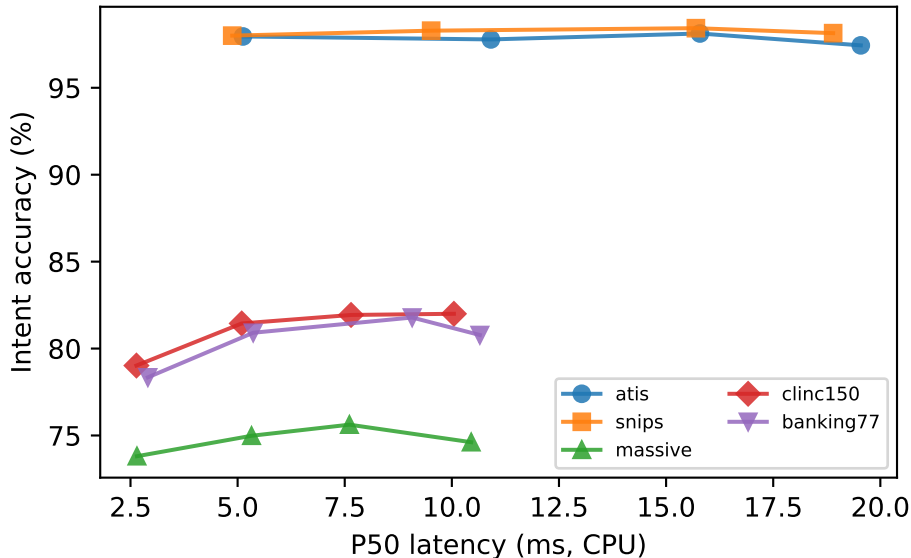
Depth Pareto: accuracy vs latency (C1)
