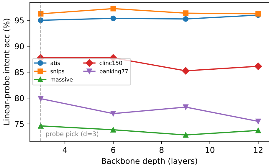
Probe accuracy saturates early (C1)
